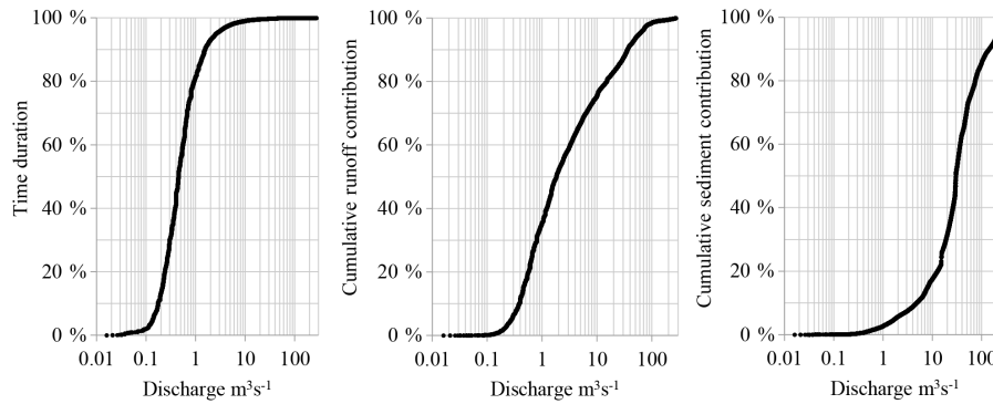
Figure 3. Cumulative frequency, water and sediment inputs assigned to ordinal discharge in the Wadi Sebdo (1973–2004).
