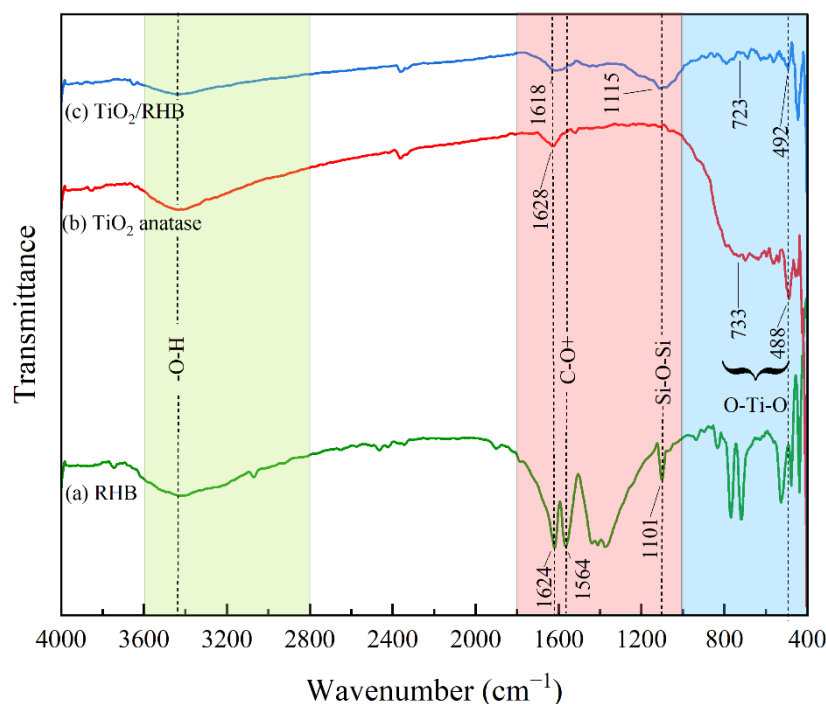
Figure 4. FTIR spectra of (a) RHB; (b) \text{TiO}_2 anatase; (c) \text{TiO}_2/\text{RHB} .
