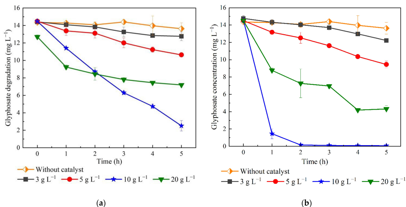
Figure 5. Glyphosate removal capacity by different catalyst dosages using (a) 9 W lamp and (b) 2 × 9 W lamps.
