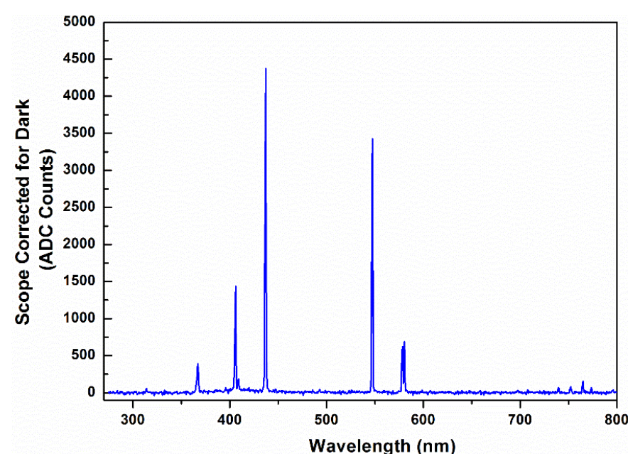
Figure A1. Irradiation spectrum of the UV lamp.
