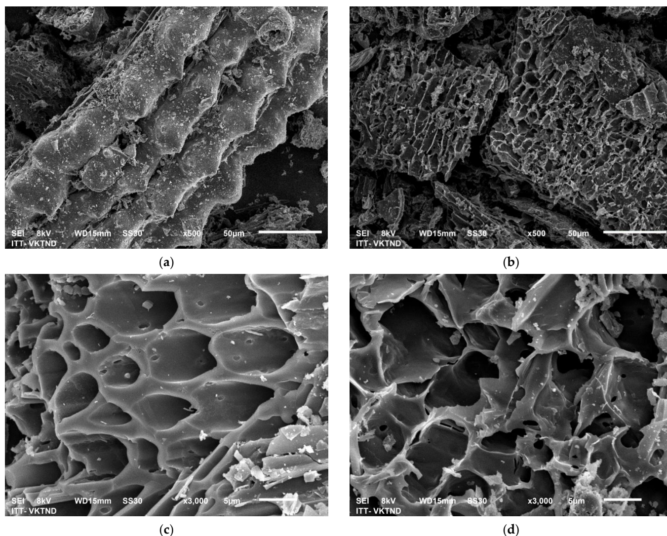
Figure 2. SEM images \text{TiO}_2 /RHB composites with different magnification at 50 \mu\text{m} (a,b) and at 5 \mu\text{m} (c,d).
