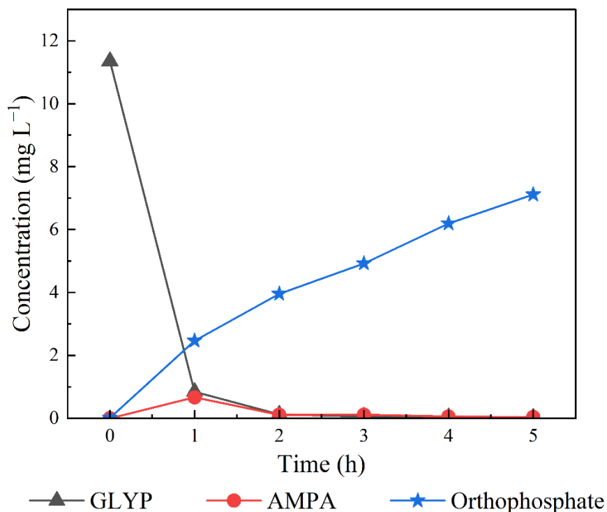
Figure 8. Photodegradation of 15 mg L -1 commercial glyphosate (pH 3.0) in the presence of 10 g L -1 TiO 2 /RHB (2 UV lamps emitting λ = 365 nm).
