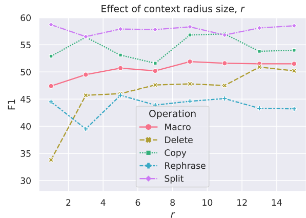
Figure 4: Effect of context window size on F1 scores.
