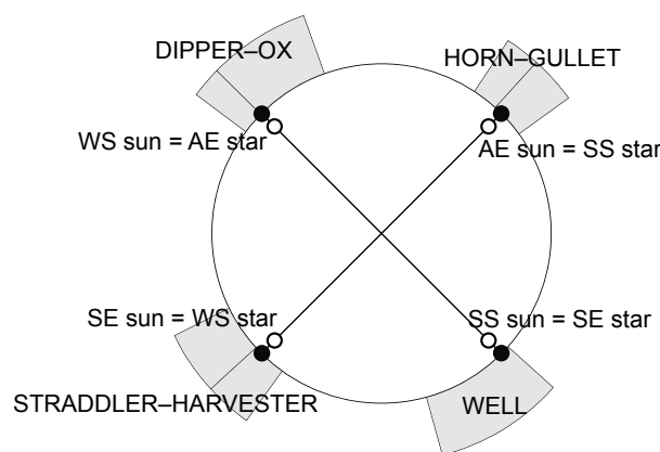
Figure 5. Illustration of Kong Yingda’s description of the position of the sun and “centered stars” in the “Yaodian”.
