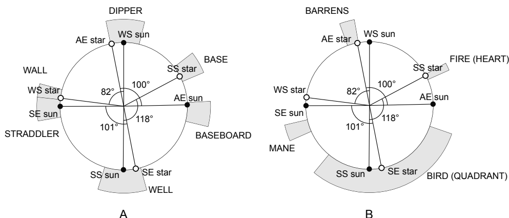
Figure 4. Distribution of solar positions and centered stars according to He Chengtian’s solar table for 443 (A) compared to the “Yaodian”, as per Liu Chunfeng’s analysis (B). As such, either the centered stars for the autumn equinox (AE) and summer solstice (SS) work, and Mane is too far east, or the winter solstice (WS) works and Barrens and Fire are too far west. Diagram based on Qu (2008, p. 188, Figure 3-14).
