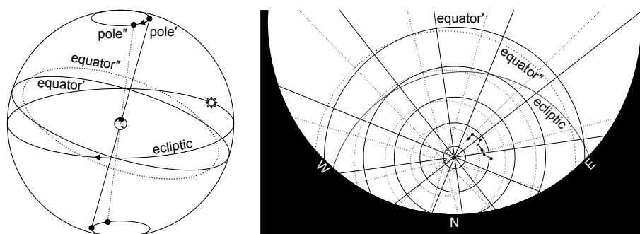
Figure 1. The Earth’s axial precession.
