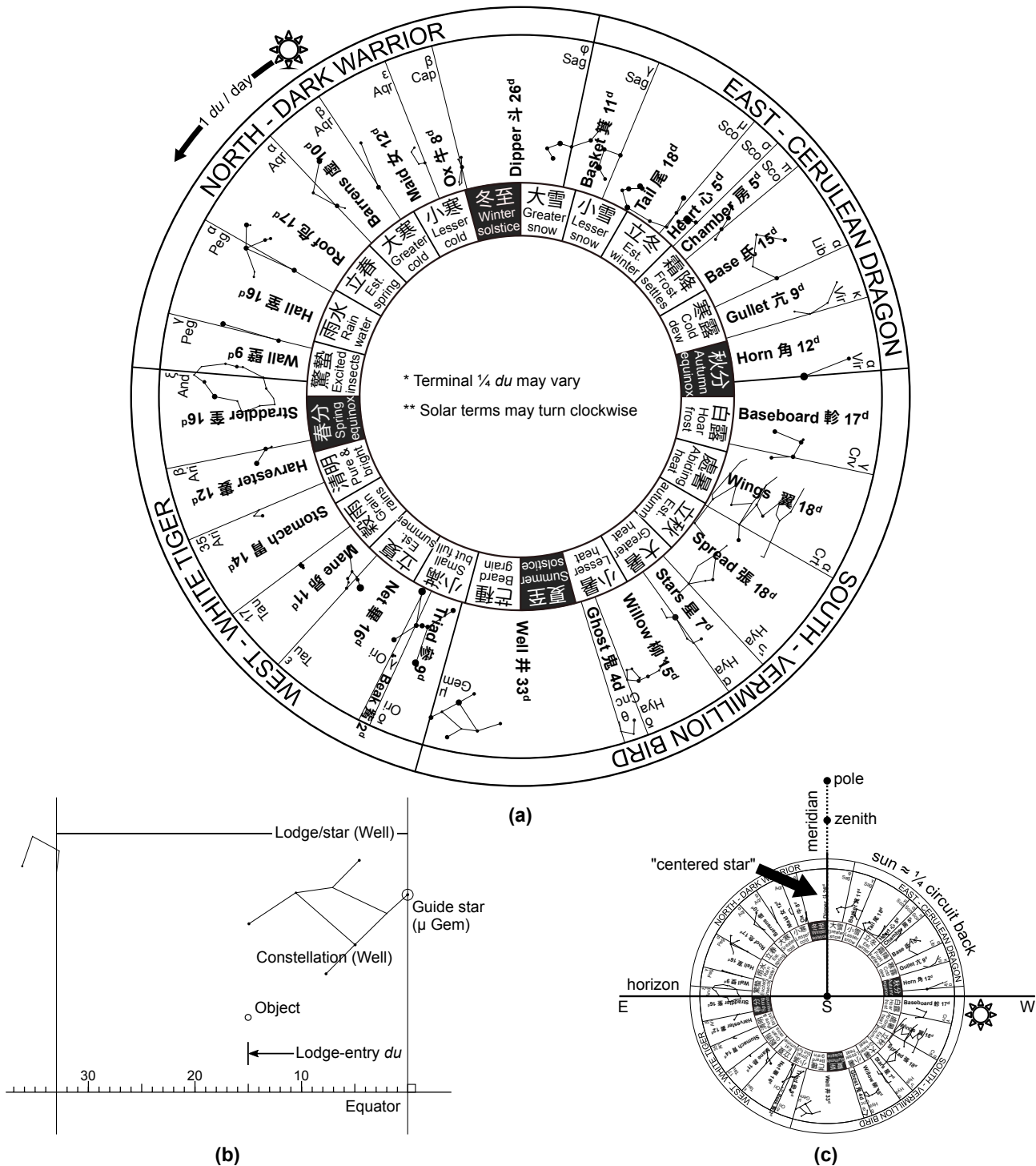
Figure 2. (a) The 28 lodges and 24 solar terms. (b) “Lodge entry-du” (ruxiu du 入宿度). (c) A “centered star” (zhongxing 中星). The du 度 is a linear measure of the circumference of an astronomical great circle defined as the daily displacement of the mean sun, meaning that there are as many du in a circle as there are days in the sidereal year and, roughly speaking, 365\frac{1}{4} du = 360^\circ , and 1 du = 0.99^\circ . The specific lodge widths and solar term association are as per He Chengtian 何承天 (370–447).
