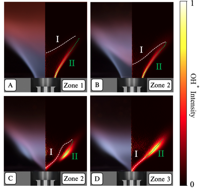
FIGURE 3: Flame images corresponding to different stabilization regimes. Left: Direct visualization in the visible band. Right: Inverse Abel transformed \text{OH}^* images. (a) Anchored flame in Zone 1. (b) Anchored flame in Zone 2. (c) Lifted flame in Zone 2. (d) Lifted flame in Zone 3. Operating conditions are given in Tab. 1.
