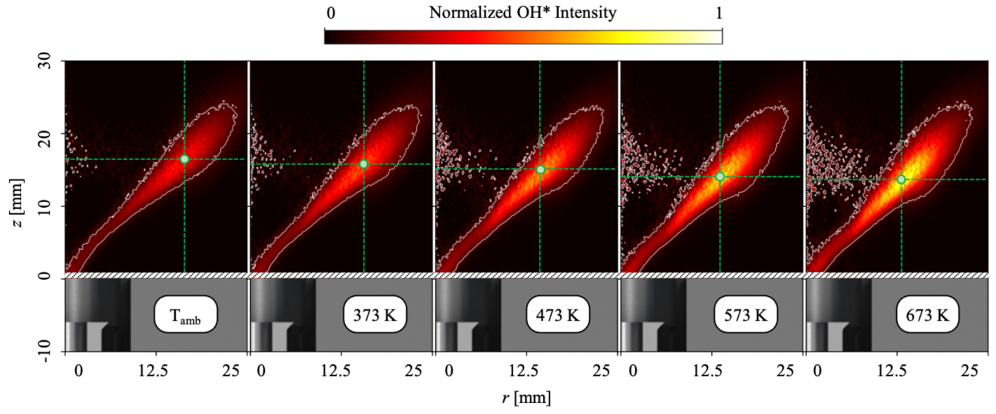
FIGURE 6: Inverse Abel transformed OH* images collected for the same input thermal power \mathcal{P}_{th} = 18 kW and same global equivalence ratio \phi_g = 0.6 and increasing air preheating temperature T_{air,in} from ambient to 673 K.
