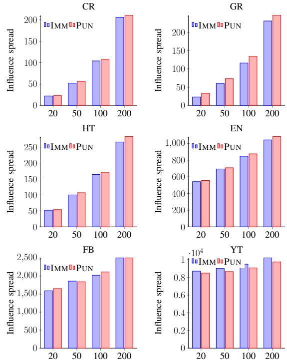
Fig. 2. PUN vs. IMM for IC with p = 0.01 .
