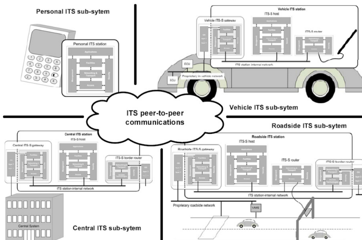
Figure 5 – type de stations de communication ITS et architecture logicielle (9)
