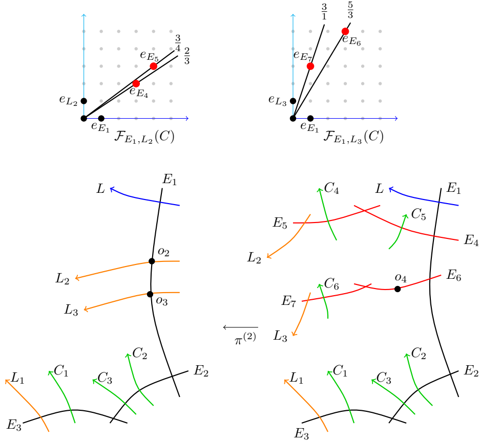
FIGURE 17. Second level of Newton modifications in Example 4.28
