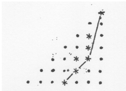
FIGURE 23. The compact sides of a Newton polygon, as represented by Cramer
