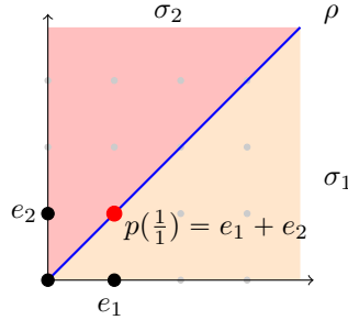
FIGURE 13. The subdivision of Example 3.27, defining the toric blow up of the origin of \mathbb{C}^2
