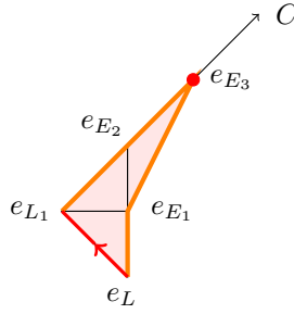
FIGURE 41. The lotus \Lambda_\pi(C) of Example 5.32
