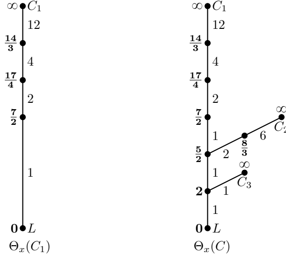
FIGURE 52. The Eggers-Wall tree of the curve singularities C_1 and C of Example 6.5
