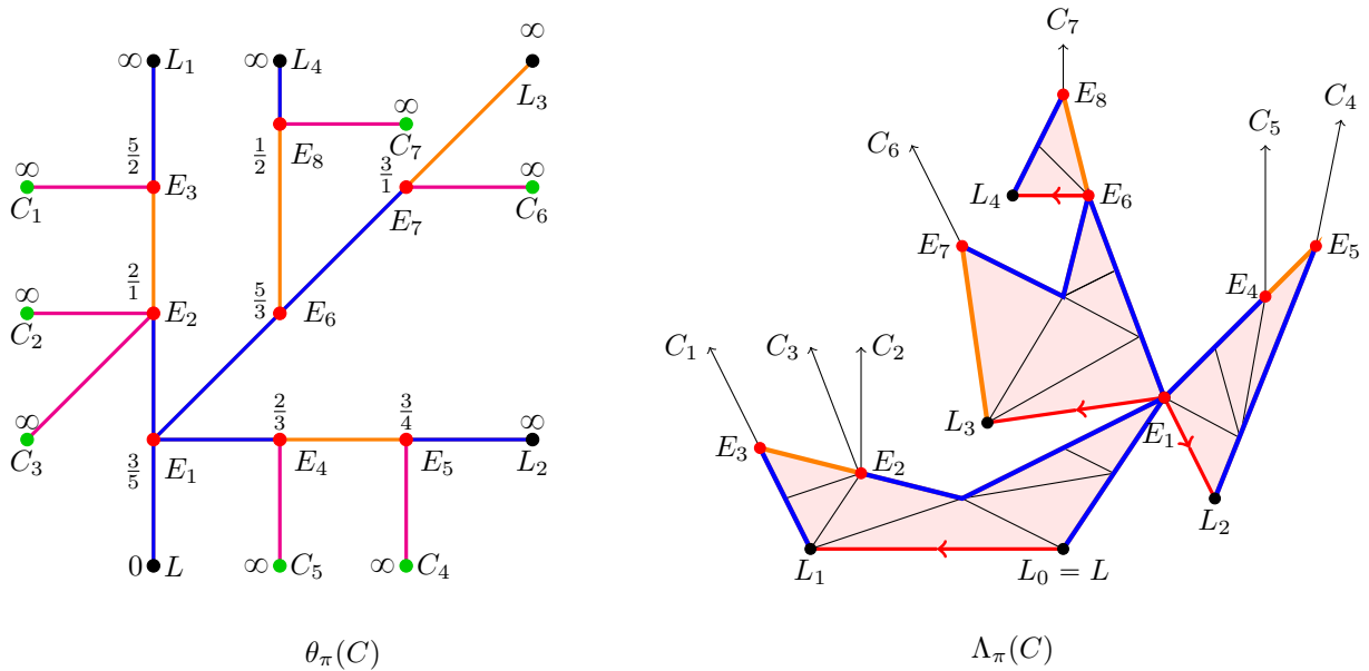
FIGURE 37. Comparison of the fan tree and the lotus of Example 5.28
