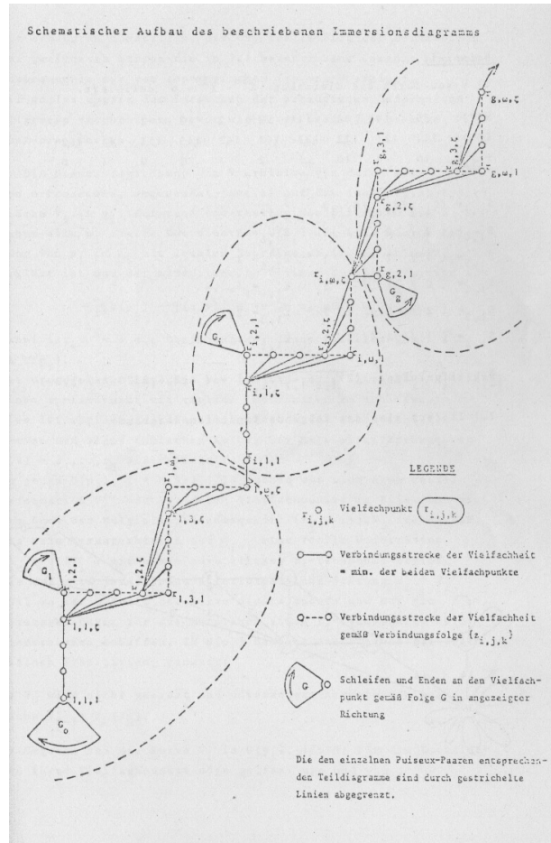
FIGURE 50. The general shape of Schulze-Röbbecke's divides
