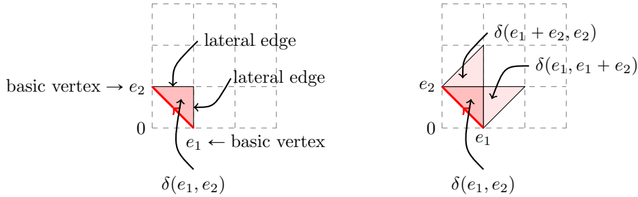
FIGURE 25. Vocabulary and notations about petals
