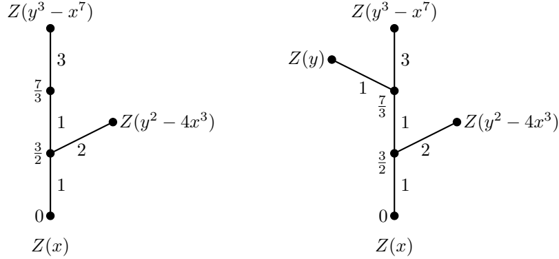
FIGURE 51. The Eggers-Wall trees of Z(f(x, y)) and Z(xy f(x, y)) from Example 6.4
