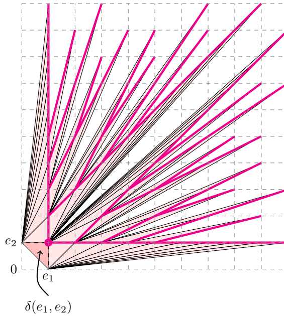
FIGURE 29. Partial view of the Enriques subtree of the universal lotus \Lambda(e_1, e_2)
