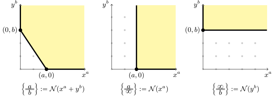
FIGURE 53. The elementary Newton polygons \left\{\frac{a}{b}\right\} , \left\{\frac{a}{\infty}\right\} , \left\{\frac{\infty}{b}\right\}
