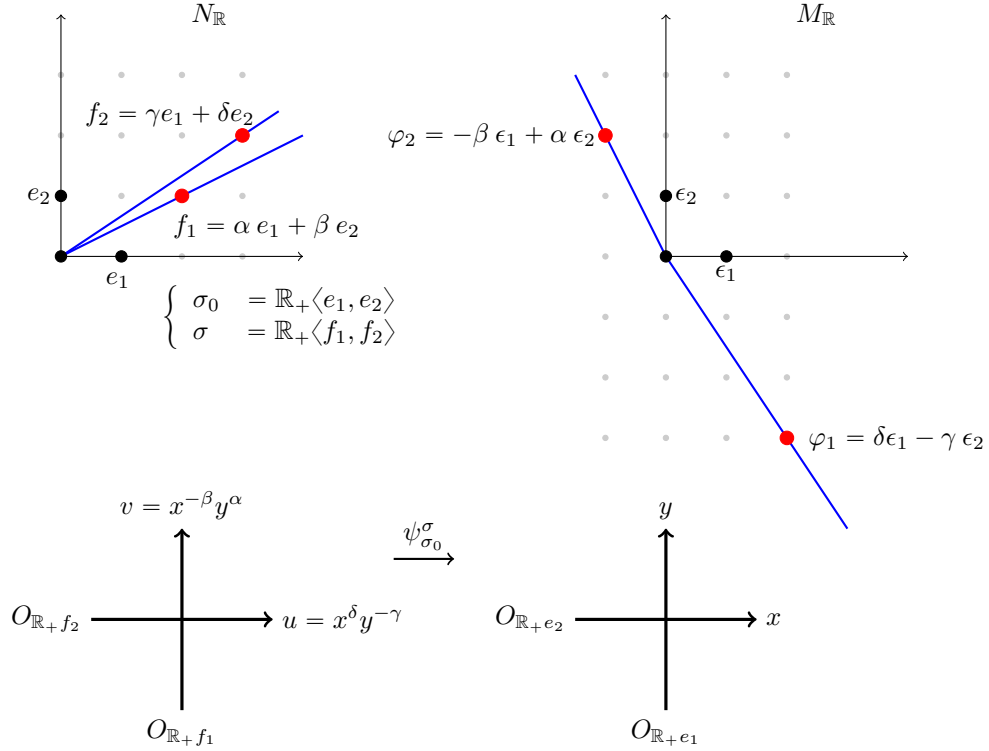
FIGURE 12. The toric morphism defined by the two regular cones of Example 3.26
