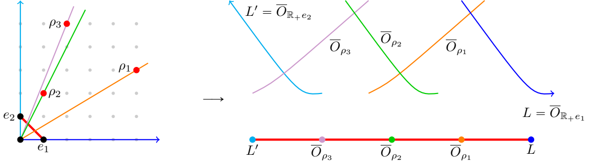
FIGURE 11. The dual graph of the total transform (\psi_{\sigma_0}^{\mathcal{F}})^{-1}(L + L')
