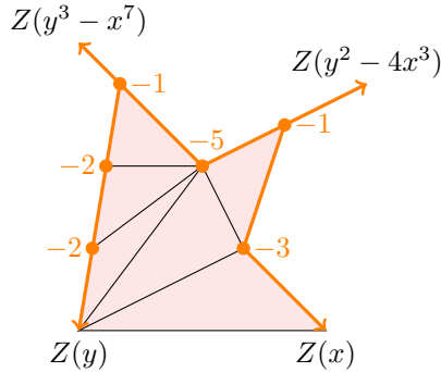
FIGURE 6. The lotus of f(x, y) = (y^2 - 4x^3)(y^3 - x^7)
