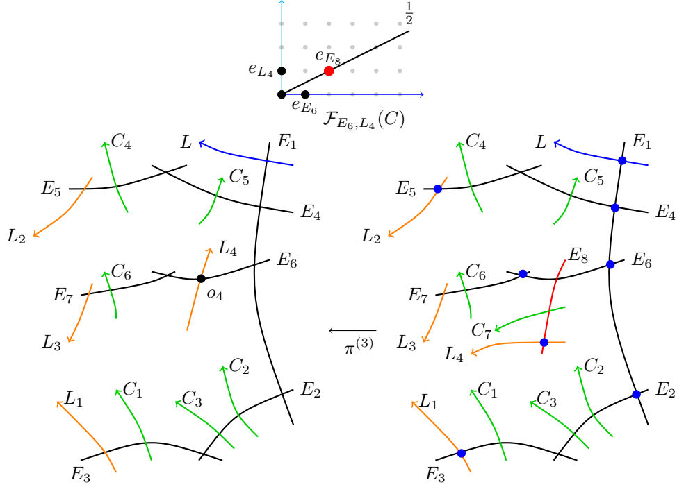
FIGURE 18. Third level of Newton modifications in Example 4.28
