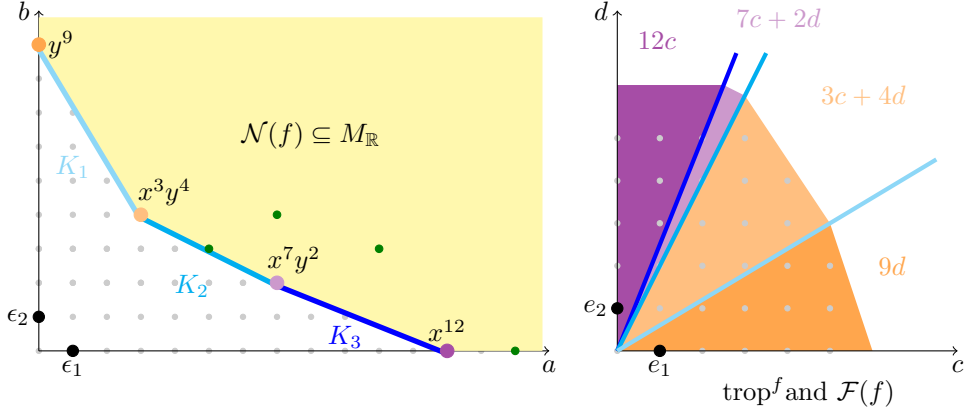
FIGURE 15. The Newton polygon, the tropicalization and the Newton fan of Example 4.10
