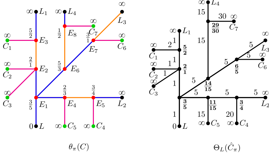
FIGURE 55. The fan tree \theta_\pi(C) and the corresponding Eggers-Wall tree \Theta_L(\hat{C}_\pi) in Example 6.29
