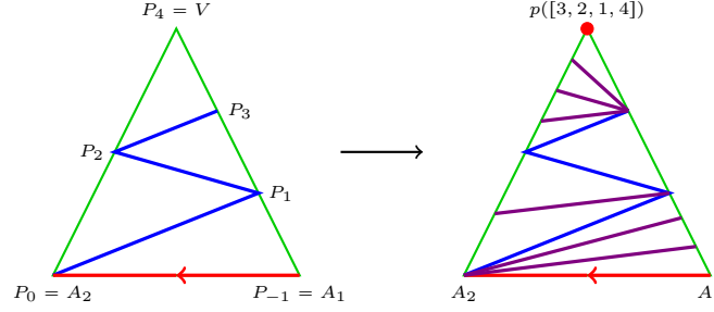
FIGURE 32. The construction of the abstract lotus \Delta([3, 2, 1, 4])
