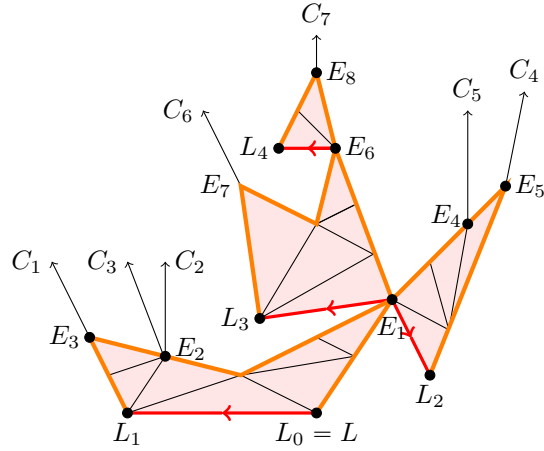
FIGURE 36. The lotus of the toroidal pseudo-resolution of Example 5.28
