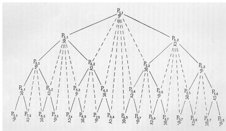
FIGURE 49. Du Val's version of universal lotus
