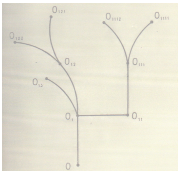
FIGURE 47. An Enriques diagram
