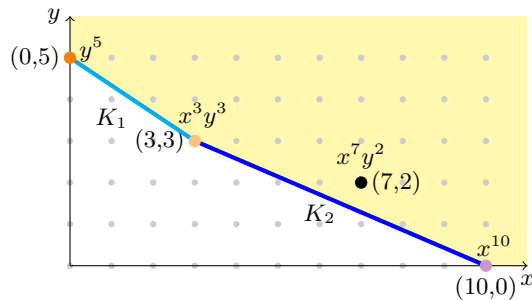
FIGURE 4. The Newton polygon of the series f(x, y) = (y^2 - 2x^3)(y^3 - x^7)
