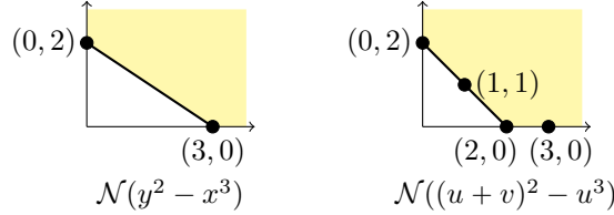
FIGURE 14. Illustration of Remark 4.3
