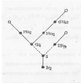
FIGURE 57. An Eggers tree
