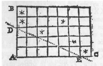
FIGURE 22. The first Newton polygon
