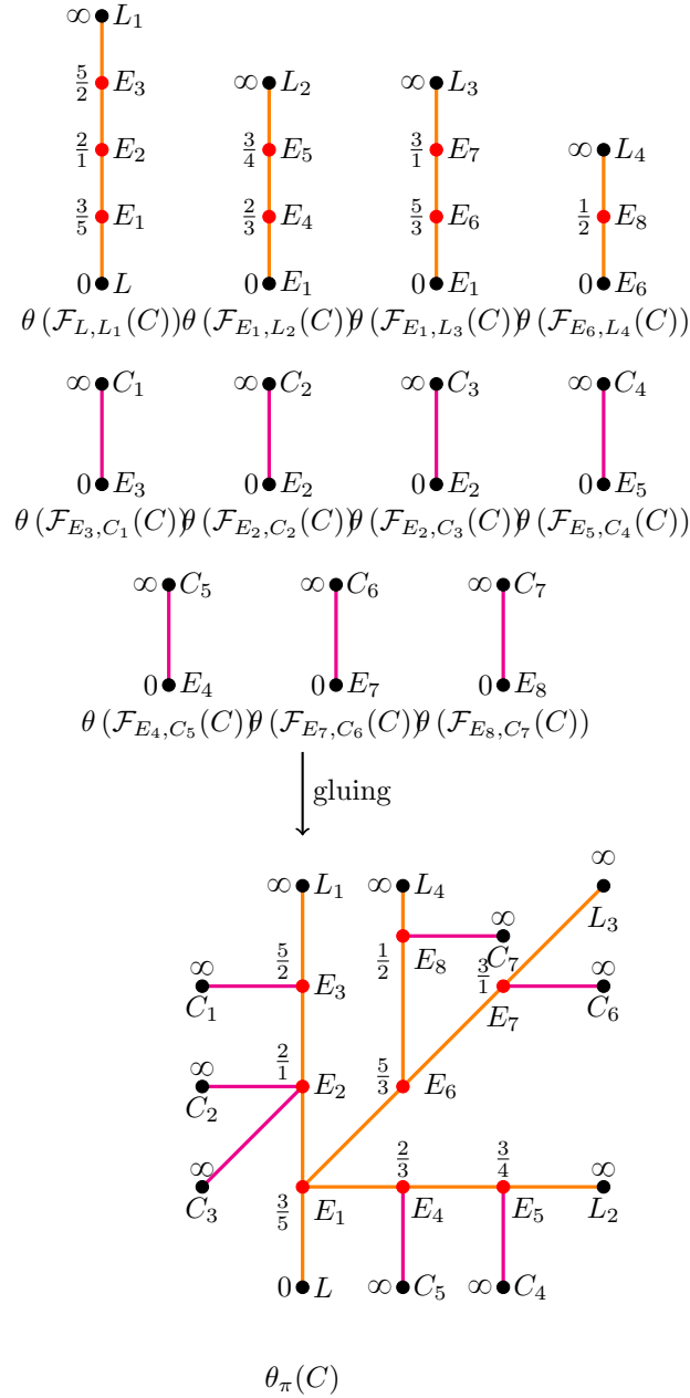
FIGURE 20. Construction of the fan tree of the toroidal pseudo-resolution of Example 4.28
