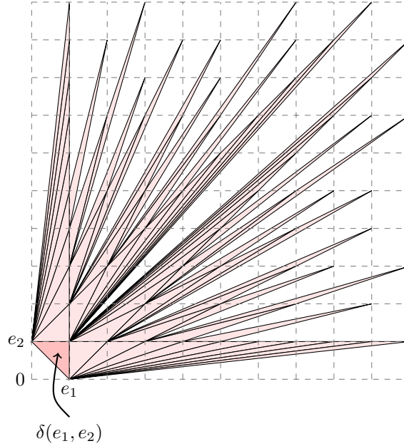
FIGURE 26. Partial view of the universal lotus \Lambda(e_1, e_2) relative to (e_1, e_2)
