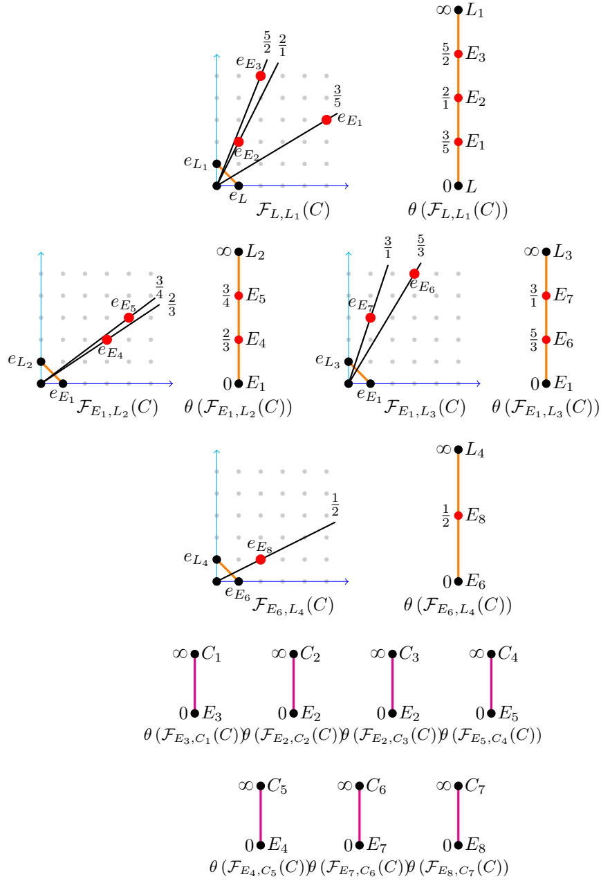
FIGURE 19. The trunks associated to the toroidal pseudo-resolution of Example 4.28
