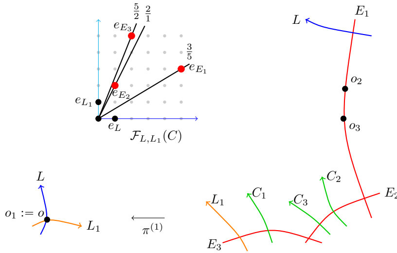
FIGURE 16. First level of Newton modifications in Example 4.28
