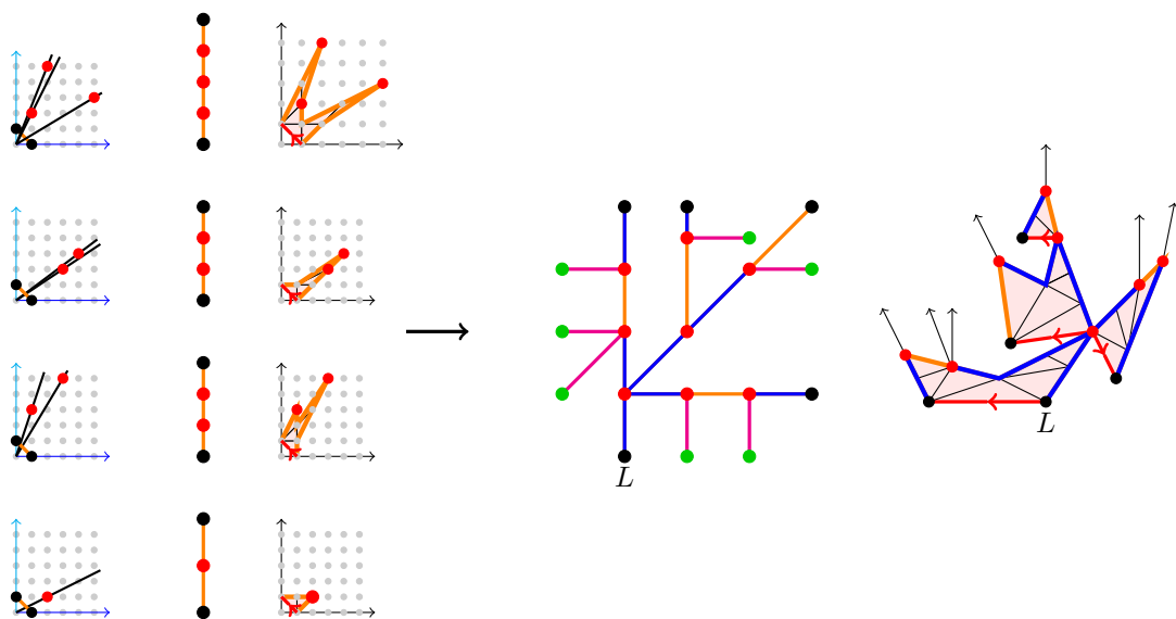
FIGURE 58. Overview of the constructions of the paper
