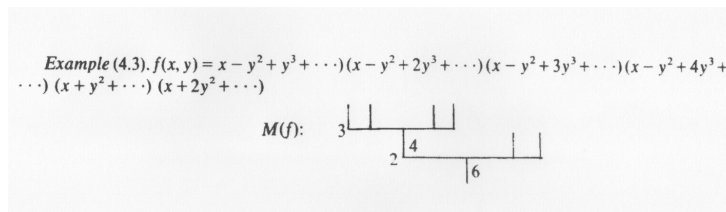
FIGURE 56. A Kuo-Lu tree
