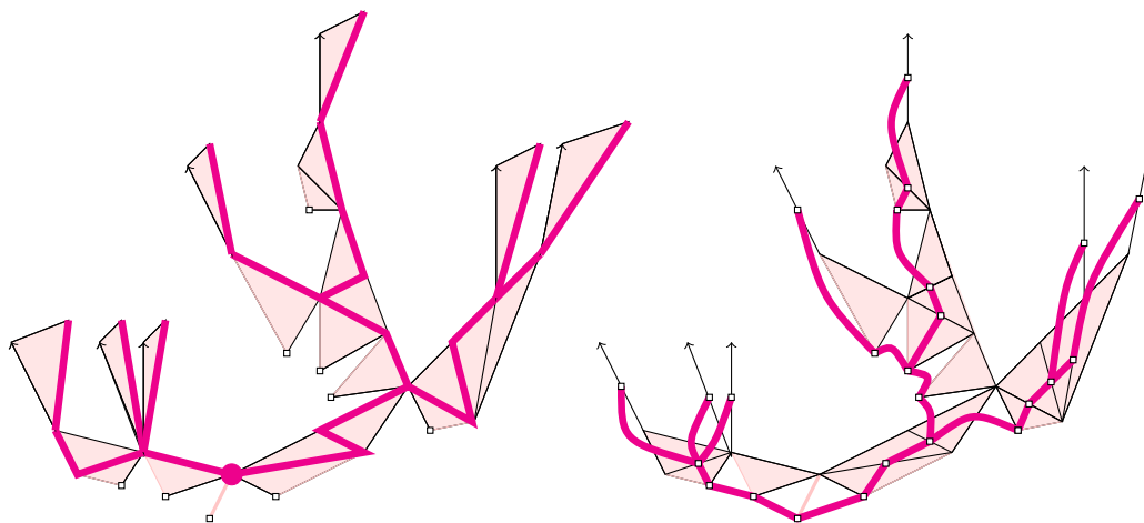
FIGURE 46. Two ways of visualizing the Enriques tree on a truncated lotus
