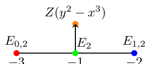
FIGURE 3. The weighted dual graph of the minimal embedded resolution of the semicubical parabola
