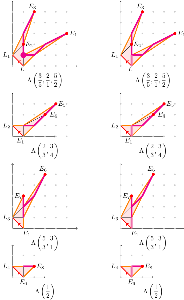
FIGURE 39. The Enriques trees and the extended Enriques trees in Example 5.31
