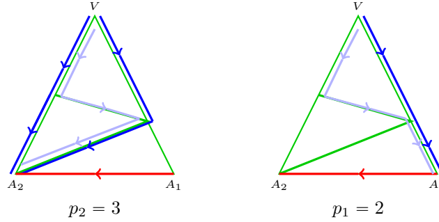
FIGURE 33. An illustration of Proposition 5.21 for p_2/p_1 = 3/2
