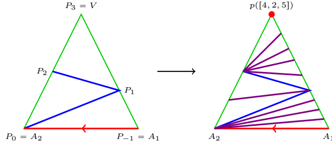
FIGURE 31. The construction of the abstract lotus \Delta([4, 2, 5])
