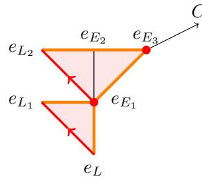
FIGURE 43. The lotus \Lambda_\pi(C) of Example 5.33
