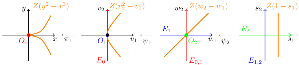
FIGURE 2. Building iteratively the minimal embedded resolution of the semicubical parabola
