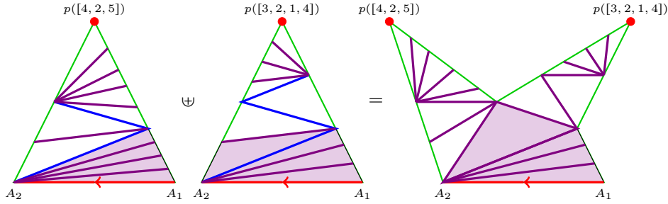
FIGURE 34. The abstract lotus \Delta([4, 2, 5], [3, 2, 1, 4])
