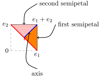
FIGURE 44. The two semipetals and the axis of the petal \delta(e_1, e_2)
