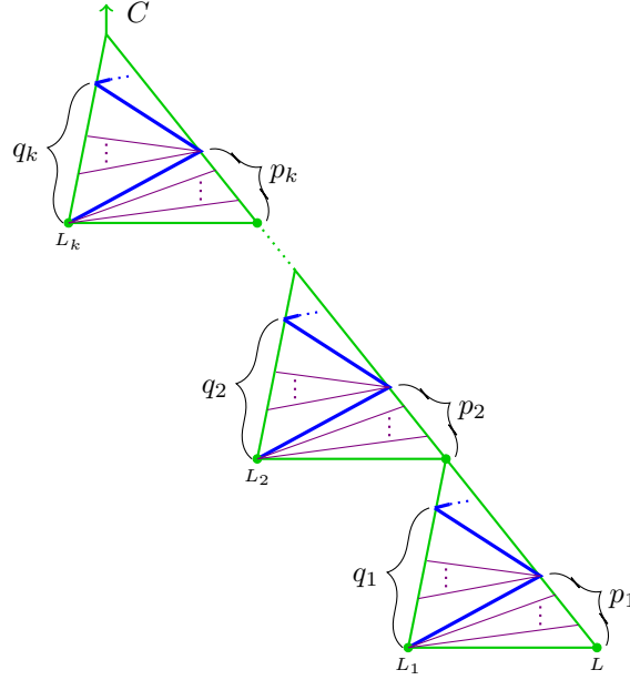
FIGURE 38. The lotus of toroidal pseudo-resolution for one branch from Example 5.30
