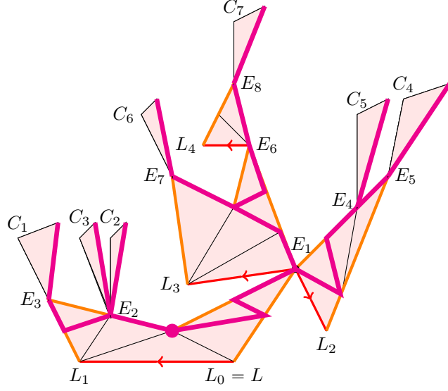
FIGURE 40. The Enriques tree of the toroidal pseudo-resolution of Example 5.31
