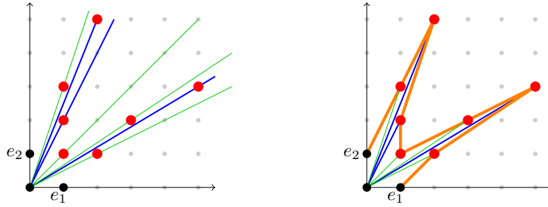
FIGURE 9. The regularization \mathcal{F}^{reg}(3/5, 2/1, 5/2) of the fan of Figure 8
