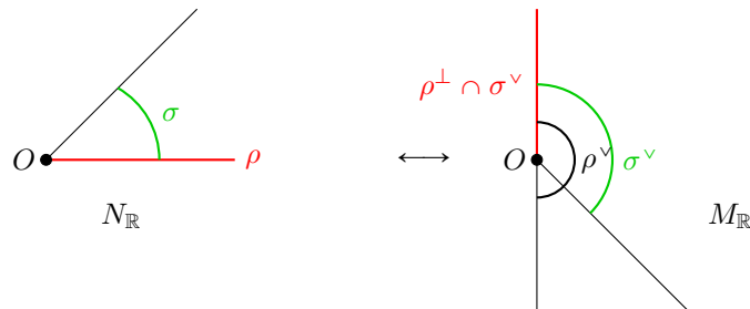
FIGURE 10. The bijection between the faces of \sigma and \sigma^\vee
