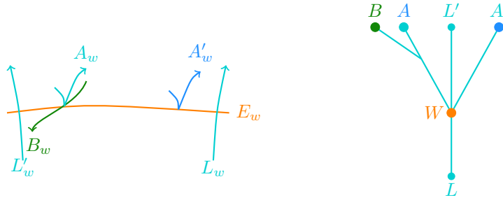
FIGURE 54. The choice of branch A' in the proof of Proposition 6.20 (2)
