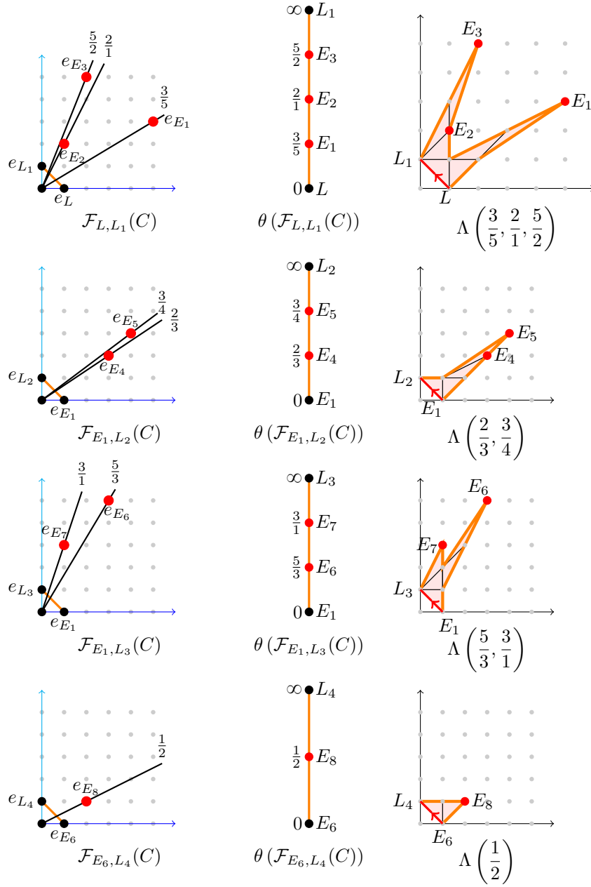
FIGURE 35. The 2-dimensional Newton lotuses of Example 5.28
