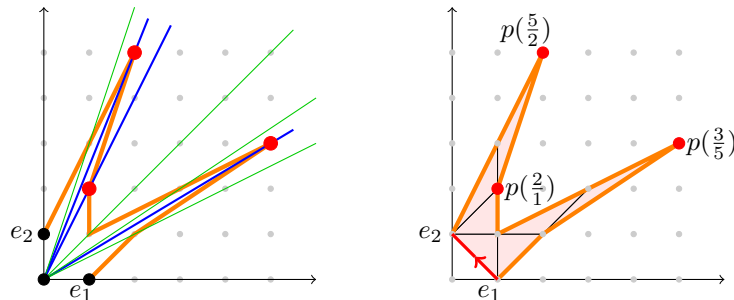
FIGURE 28. The regularized fan \mathcal{F}^{reg}(3/5, 2/1, 5/2) and the Newton lotus \Lambda(3/5, 2/1, 5/2)
