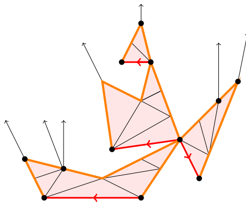
FIGURE 1. A lotus. It is part of Figure 36, which corresponds to Example 5.28.
