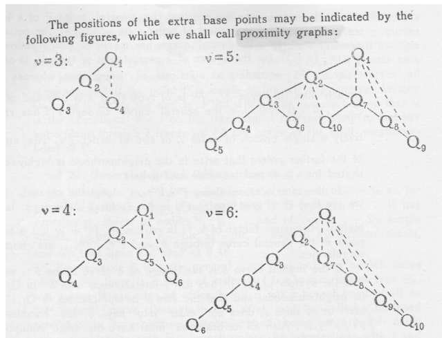
FIGURE 48. Du Val's "proximity graphs"
