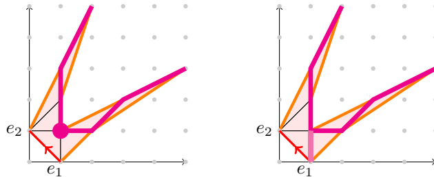
FIGURE 30. The Enriques tree and the extended Enriques tree of the lotus \Lambda(3/5, 2/1, 5/2)
