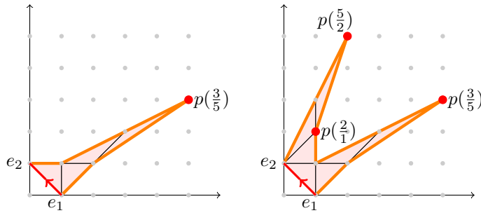
FIGURE 27. The Newton lotuses \Lambda(3/5) , \Lambda(3/5, 2/1, 5/2) and their marked points
