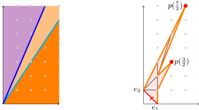
FIGURE 5. The Newton fan of f(x, y) = (y^2 - 4x^3)(y^3 - x^7) and its associated lotus
