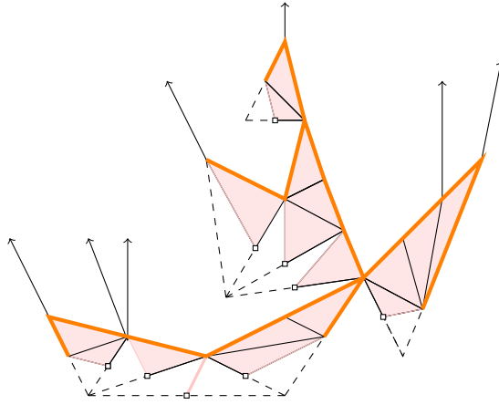
FIGURE 45. The truncation of the lotus of Figure 36 (see Example 5.36)
