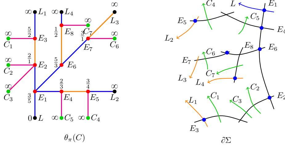
FIGURE 21. The fan tree \theta_\pi(C) is isomorphic to the dual graph of the toroidal boundary \partial\Sigma
