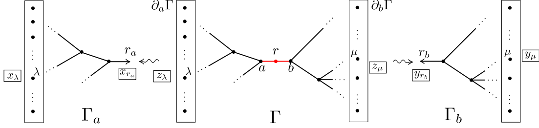
FIGURE 4. Splitting the splice diagram \Gamma along any interior point r on the central edge [a, b] yields the diagrams \Gamma_a and \Gamma_b , with roots r_a and r_b , respectively. The variables associated to the leaves on each diagram are labeled from left to right by x_\lambda , z_\lambda , z_\mu and y_\mu , respectively.
