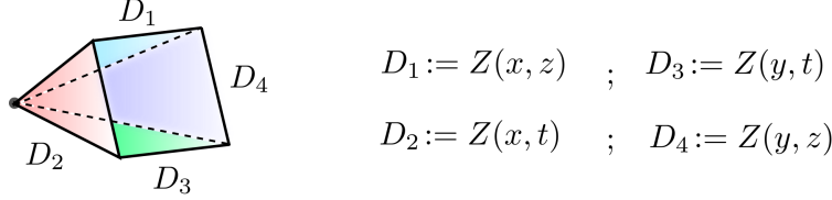
FIGURE 10. Boundary strata of the toroidal variety (W, \partial W) , where W := Z(xy - zt) \subset \mathbb{C}^4 . The toric boundary \partial W has four irreducible components (see Example 4.7).
