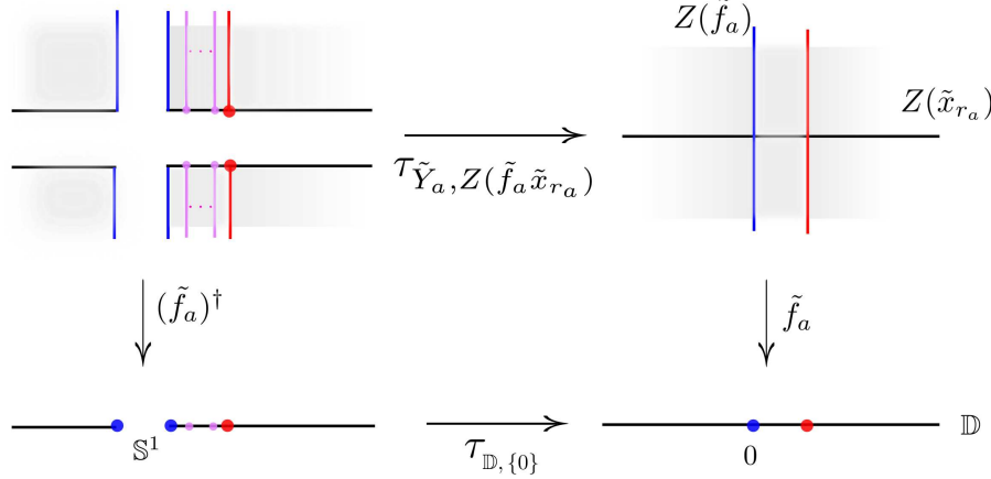
FIGURE 9. Local drawing of the rounding operation away from \tilde{X}_a . The canonical representative of the Milnor fiber (in red) has been cut using Z(\tilde{x}_{r_a}) . The special fiber Z(\tilde{f}_a) is drawn in blue. The origin has been replaced by the circle \mathbb{S}^1 under the real oriented blow up \tau_{\mathbb{D}, \{0\}} of Subsection 4.2. This circle is depicted on the left as a pair of points. The two remaining fibers (in purple) indicate the local triviality of the Milnor fibration.
