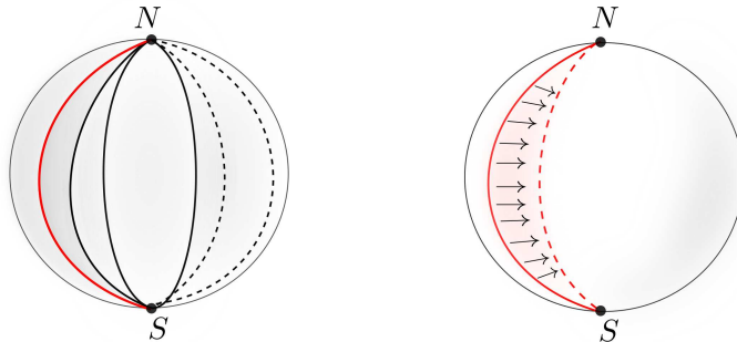
FIGURE 5. From left to right: collection of meridians forming an open book on the sphere \mathbb{S}^2 with a distinguished page (in red), and pushing of this page inside the interior of the ball bounded by \mathbb{S}^2 , featured as a dashed arc. The binding is given by the north and south poles.
