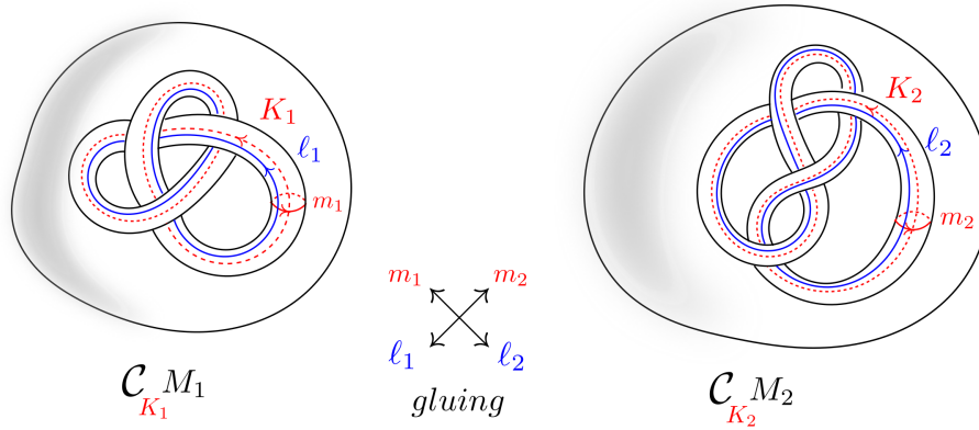
FIGURE 1. Splicing the integral homology spheres M_1 and M_2 along the knots K_1 and K_2 (see Definition 2.21).
