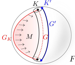
FIGURE 7. A tubular neighborhood of G inside F , and copies G' (in blue) and G_K (in red) of G (in dashed red) with G_K \subset \partial_{top} F satisfying \partial_{top} G = \partial_{top} G_K = K and \partial_{top} G' = K' . The pink shaded area M bounded by G_K and G avoids G' (see the proof of Proposition 2.45).
