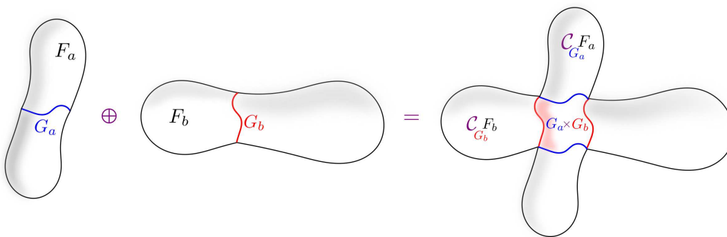
FIGURE 6. Splicing of two four-dimensional manifolds F_a and F_b with integral homology sphere boundaries along properly embedded surfaces called G_a and G_b , respectively (see Definition 2.44 ).
