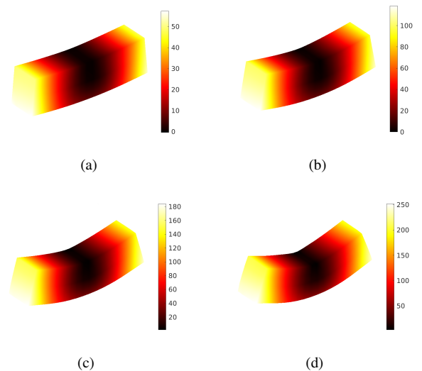
Figure 12: Initialization results in terms of displacements (expressed in voxels, 1 \text{ vx} \equiv 0.1 \text{ mm} ) along the z ( i.e. , vertical) direction for the different deformed configurations. (a) 5 mm, (b) 10 mm, (c) 15 mm and (d) 20 mm deflections
