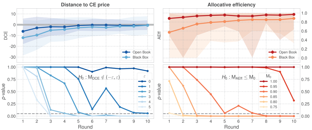
NOTES: Top: Left. DCE with a one-standard-deviation interval around the average per round (blue shade) evolving over time. Right. AEff with an interval indicating the least and the most efficient markets around it (red shade) over time. Bottom: p -Values corresponding to the hypothesis tests pooling across all (Open Book and Black Box) treatments. The horizontal dashed lines indicate the 0.05 significance level. Left. Convergence to CE price range. Right. Convergence to allocative efficiency.
