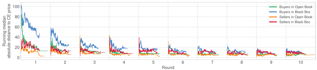
NOTES: The median absolute bid/ask distances to CE are calculated across all experimental sessions using sliding windows of size 100 (at the outset of each round, the minimum window size is set to 5). Specifically, all Open Book/Black Box bid/ask distances to CE are sorted by trading round T and time t_T , and, for time t_T , the median distance is computed by taking into account the distance at time t_T and the most recent 99 distances preceding it in the trading round T under observation. If there are strictly less than 99 but at least four distances preceding it, all of these are taken into account. Otherwise, the median value is not computed.
