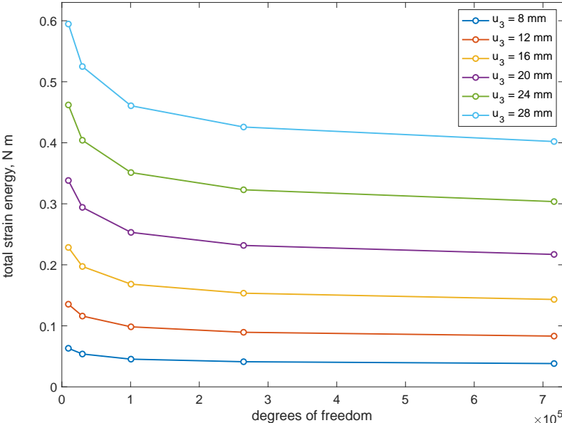
Figure 14: Convergence plots.
