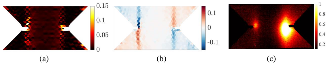
Fig. 14 Measured strain and temperature fields for the first cycle peak (289 MPa). (a) \epsilon_{yy} , (b) \epsilon_{xy} and (c) \Delta T = T - T_3 (in °C).
