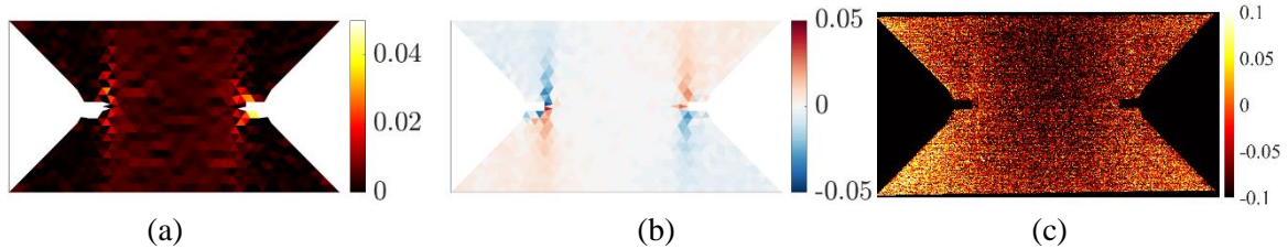
Fig. 5 Measured strain and temperature fields for the first cycle peak (145 MPa). (a) \varepsilon_{yy} , (b) \varepsilon_{xy} and (c) \Delta T = T - T_1 (in ^{\circ}\text{C} ).
