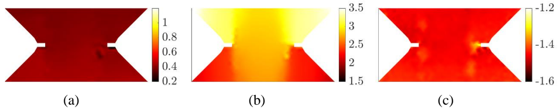
Fig. 16 Measured displacement fields expressed in mm for the fifth cycle peak (262 MPa). Components U_x (a), U_y (b) and U_z (c).
