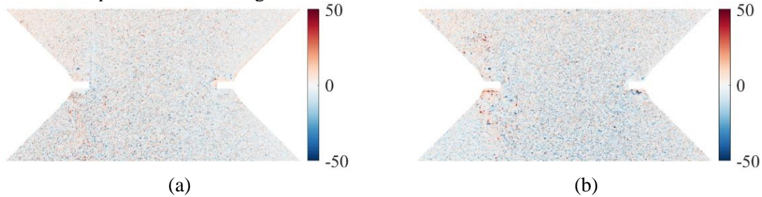
Fig. 9 Gray level residuals for the second cycle peak (196 MPa) for the first (a) and second (b) cameras.
