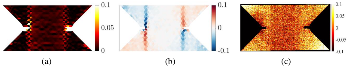
Fig. 11 Measured strain and temperature fields for the first cycle peak (245 MPa). (a) \varepsilon_{yy} , (b) \varepsilon_{xy} and (c) \Delta T = T - T_2 (in ^{\circ}\text{C} ).
