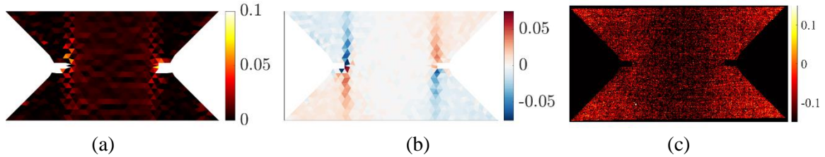
Fig. 8 Measured strain and temperature fields for the first cycle peak (196 MPa). (a) \varepsilon_{yy} , (b) \varepsilon_{xy} and (c) \Delta T = T - T_2 (in ^{\circ}\text{C} ).
