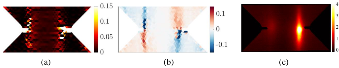
Fig. 17 Measured strain and temperature fields for the first cycle peak (262 MPa). (a) \varepsilon_{yy} , (b) \varepsilon_{xy} and (c) \Delta T = T - T_4 (in ^{\circ}\text{C} ).
