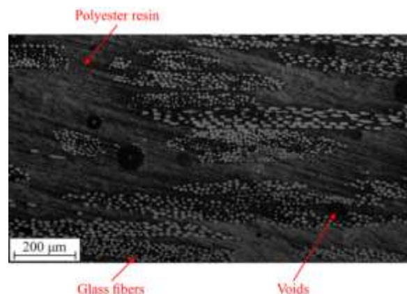
Fig. 1 Optical micrograph of the glass fiber mat reinforced polyester resin composite studied herein
