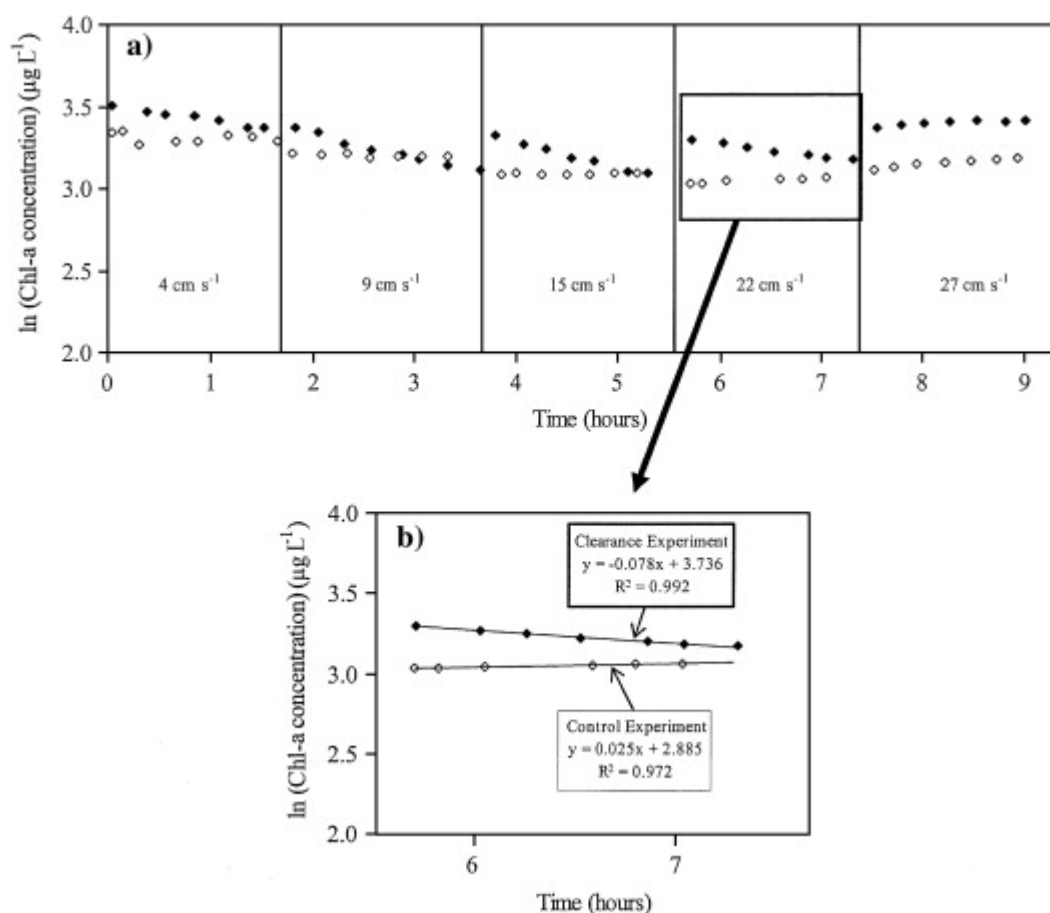
Figure 3: a) Variation with time of \ln (Chl a concentrations ( \mu\text{g}\cdot\text{l}^{-1} )) estimated from in vivo fluorescence during the clearance (Exp 1 with Lanice conchilega , \blacklozenge ) and the control (without L. conchilega , \diamond ) experiments. Flow velocity was increased from 4 to 27 \text{cm}\cdot\text{s}^{-1} every 1h45 minutes. The sharp concentration changes observed during clearance experiment are consecutive to algal concentration readjustment performed for each velocity increase (see text). b) Detailed view of the changes recorded at 22 \text{cm}\cdot\text{s}^{-1} , with linear fit and corresponding slopes (also see Table II)
