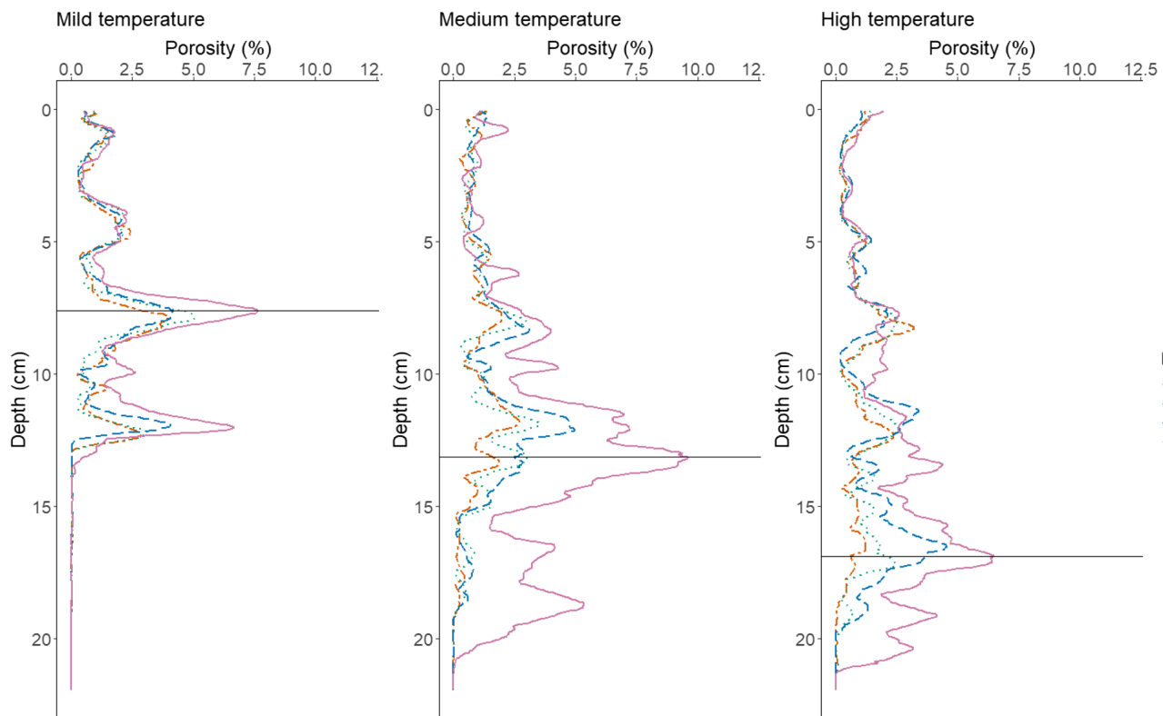
FIGURE 3 Mean porosity profiles (percentage of the empty volume compared to soil volume) per treatment. Colours and line types correspond to dates. Black horizontal lines indicate the point of maximal porosity on Day 88.
