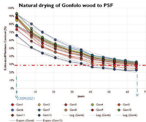
Figure 12: Moisture loss tracking curves of Gonfalo ( Q. rosea ) wood (Cayenne) [10]
