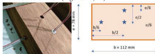
Figure 13: Natural drying - Geometry, sensor position
