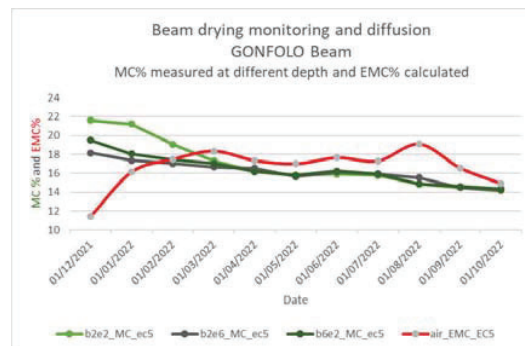
Figure 14: Moisture content (MC, %) tracking curves of Gonfalo ( Q. rosea ) wood drying – equilibrium moisture content (EMC, %) calculated from local air sensor data.
