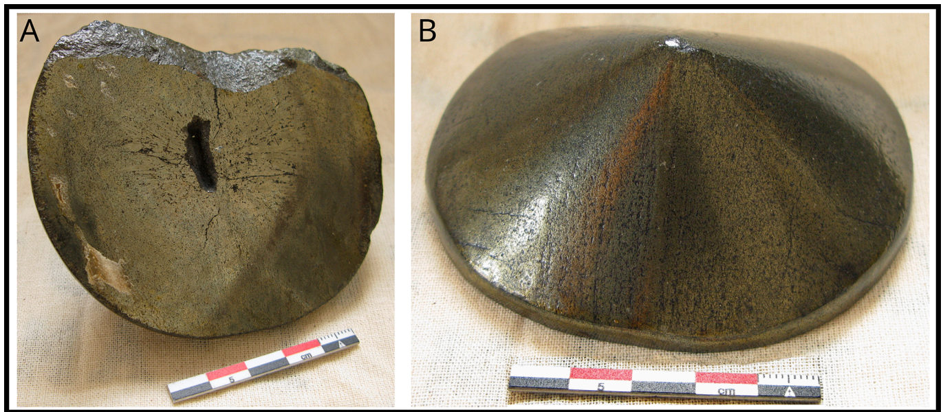
Fig. 2. A and b: a) Pyrite “Inca mirror” no. 105.504 (no.2) conserved in the Mineralogy’s collections of the MNHN seen from its basal reflective face and conic side (height: 39.8 mm; Ø base: 95.3 x 75 mm; weight: 514 g). On the conic side, the parallel striations visible between the base and the top are due to the “triglyph” twin system (Photographs F. Gendron/MNHN).
