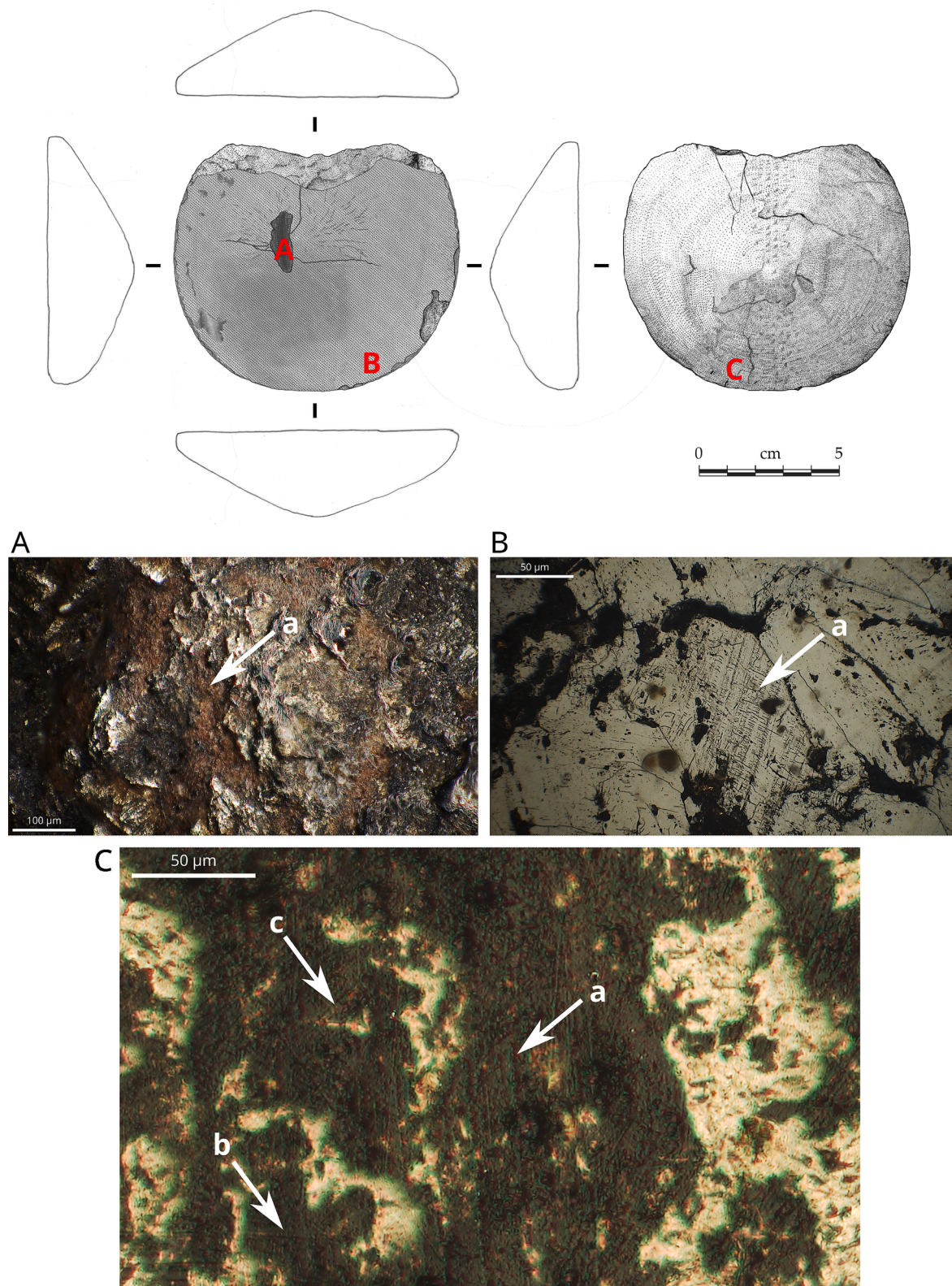
Fig. 5. Drawing of the faces and profiles of the « Inca mirror » 105.504 (no.2; Drawings É. Ahmed-Delacroix). A) image made with the MXB-5000REZ lens Middle Range at x400, scale = 100 μm, a) bottom of vacuoles filled with red powdery clusters. B) image made with MXB-5000REZ lens High Range at x1000, scale = 50 μm, unidirectional cluster of parallel glossy striations surrounded by lustrous surfaces. C) image made with the MXB-5000REZ lens Middle Range at x1000, scale = 50 μm, a) group of vertical parallel striations (≈1 to 4 μm), b) group of horizontal parallel striations and c) diagonal striations, remnants of shaping by direct polishing on a milling stone (sandstone?); (Photography A. Borel/MNHN). (For interpretation of the references to color in this figure legend, the reader is referred to the web version of this article.)
