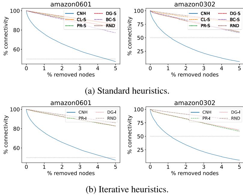
Fig. 2. Real-world product-co-purchase (PCP). Trend of graph connectivity with respect to the number of removed nodes for real-world PCP graphs using the standard and iterative strategies. The connectivity is the percentage of the initial connectivity of the graph, whereas the number of removed nodes is the percentage of the initial nodes in the graph. The horizontal gray dotted line denotes the 50% of residual connectivity.
