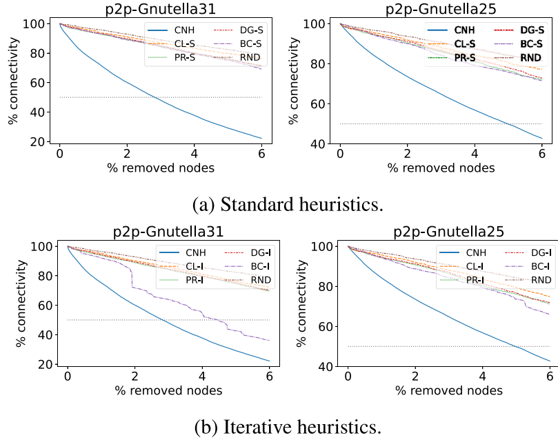
Fig. 3. Real-world peer-to-peer (P2P). Trend of graph connectivity with respect to the number of removed nodes for real-world P2P graphs using the standard and iterative strategies. The connectivity is the percentage of the initial connectivity of the graph, whereas the number of removed nodes is the percentage of the initial nodes in the graph. The horizontal gray dotted line denotes the 50% of residual connectivity.
