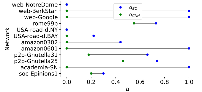
(b) \alpha_{CNH} vs. \alpha_{BC} for our real-world graphs.
