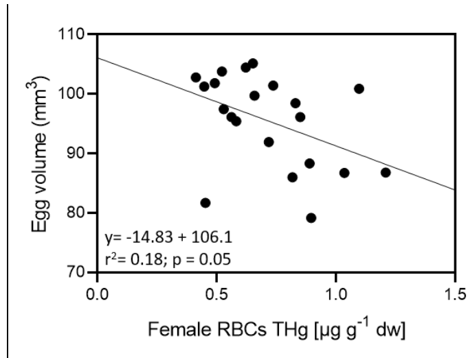
Figure 3. Relationships between red blood cells THg concentrations ( \mu\text{g g}^{-1} dw) and egg volume ( \text{mm}^3 ) of female brown skuas ( Stercorarius antarcticus ) at Esperanza/Hope Bay, Antarctic Peninsula ( 63^{\circ}24'S , 57^{\circ}01'W ) in the 2018/19 and 2019/20 breeding seasons.
