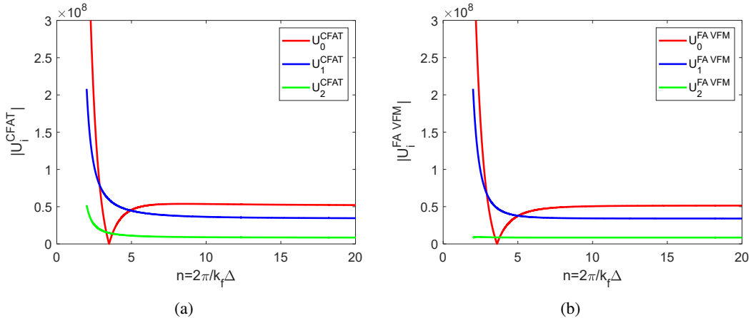
Figure 9: (a) U_0^{CFAT} , U_1^{CFAT} and U_2^{CFAT} as a function of n = \frac{2\pi}{k_f\Delta} , (b) U_0^{FA VFM} , U_1^{FA VFM} and U_2^{FA VFM} .
