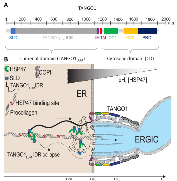
Figure 1: Model of procollagen transport by TANGO1. A. TANGO1 is a long protein that contains an ~1000 residue long intrinsically disordered TANGO1 LUM IDR in the ER lumen, an intra-membrane domain (IM) followed by a trans-membrane domain (TM) and two coiled-coil regions on the cytosolic side (CC1 and CC2). An SH3-like domain (SLD) is located at the N-terminus. B. The C-terminal cytosolic coiled-coil regions of TANGO1 were suggested to open a tunnel between the ER lumen and the ERGIC. The luminal portion of TANGO1 could separate the luminal content of the ER and the ERGIC, creating a gradient of HSP47 and pH between the ER lumen and the tunnel. Some TANGO1 LUM SLDs can bind to HSP47, which in turn binds to triple helical procollagen-generating a mechanical link that exert a force on procollagen. Because of the molecular gradients, this force is asymmetrical and drives procollagen movement. HSP47-binding sites are located per pair every ~10 nm on the procollagen. All quantities are defined along the x-axis representing the center of the tunnel. The junction between the tunnel and the ER is placed at x=0; x<0 is in the lumen of the ER and x>0 is in the tunnel towards the ERGIC. Gradients of pH and [HSP47] are maintained, possibly by a network of TANGO1 LUM IDRs.
