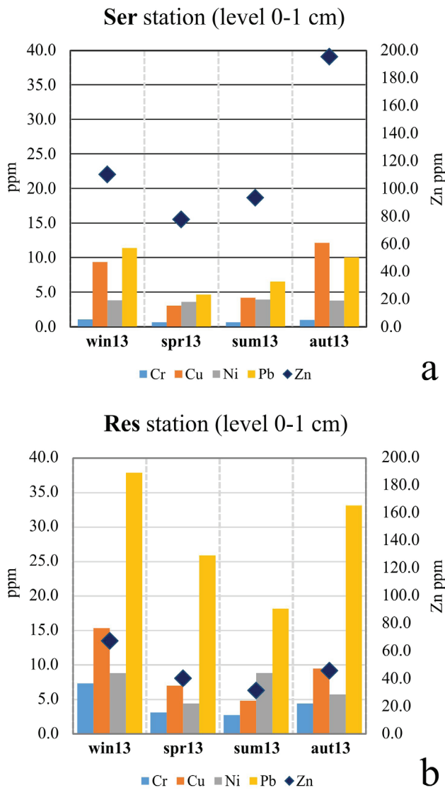
Fig. 3: Potentially toxic elements (PTE) concentration in the Ser (a) and Res (b) stations calculated for the 0-1 cm level. PTEs are expressed in micrograms per gram ( \mu\text{g/g} ).
