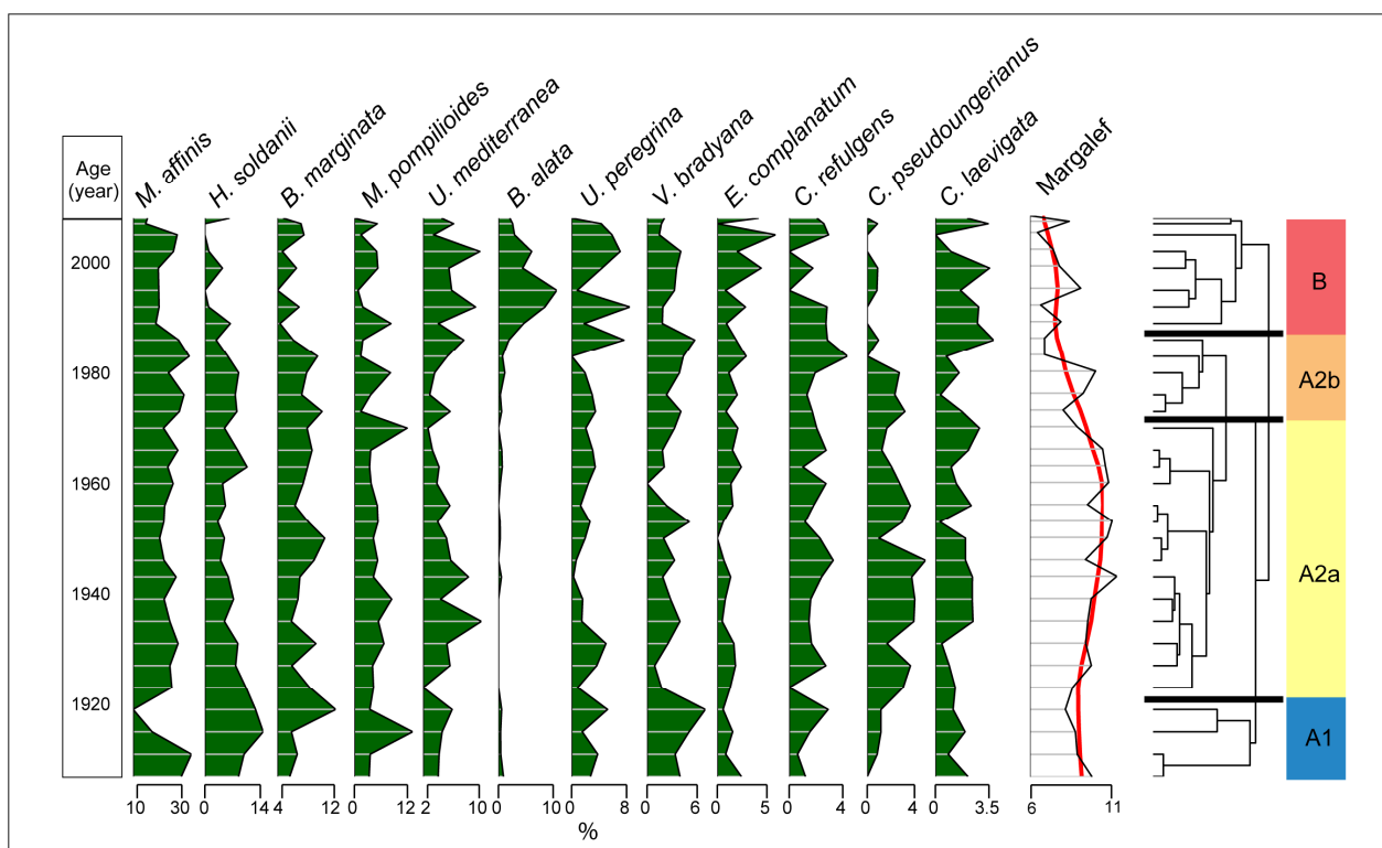
Figure 3. Hierarchical cluster analysis coupled with the plot of the relative abundance of foraminiferal taxa and the Margalef index along the different identified intervals (A1: 1907–1919; A2a: 1923–1970; A2b: 1973–1986; and B: 1989–2013) of the A2TM core. The red line represents the smoothed (5-point moving average) temporal variation of the Margalef index.
