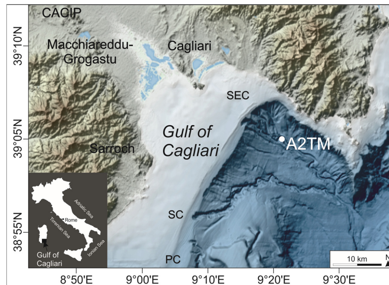
Figure 1. Map of the Gulf of Cagliari with the location of A2TM core in the Sant’Elia-Foxi canyon (SEC) along with the position of Sarroch Canyon (SC), Pula Canyon (PC), and Industrial Provincial Consortium of Cagliari (CACIP); modified after [6].
