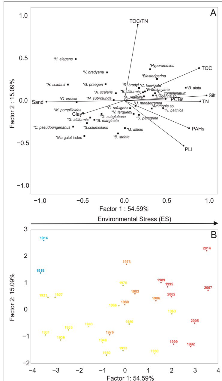
Figure 4. (A) R-mode and (B) Q-mode principal component analysis (PCA). Grain size parameters and geochemical indices are used as primary variables, and the relative abundance of benthic foraminiferal indices and Margalef index are used as secondary variables. The colour of the layers reflects the identified intervals (A1: 1907–1919—blue; A2a: 1923–1970—yellow; A2b: 1973–1986—orange; B: 1989–2013—red) by the Hierarchical cluster analysis along the A2TM core. The asterisk (*) marks the secondary variables used in the PCA.
