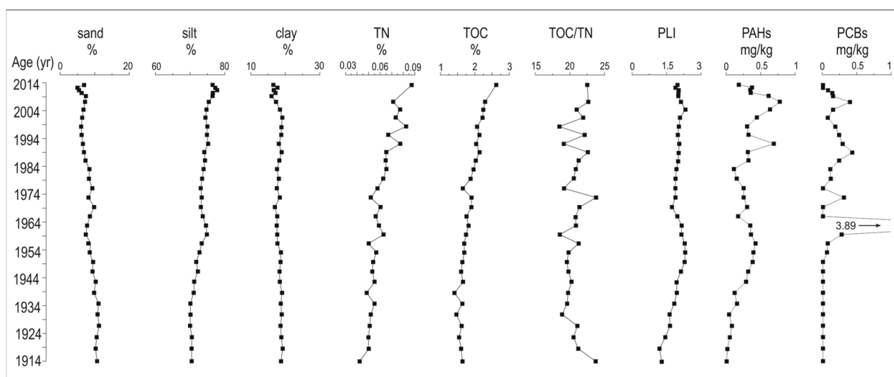
Figure 2. Grain size (i.e., sand, silt and clay and sand data from [6]), organic matter (TN: total nitrogen; TOC: total organic carbon; TOC/TN ratio) and geochemical (Pollution Load Index: PLI, Polycyclic Aromatic Hydrocarbons: PAHs; Polychlorinated Biphenyls: PCBs; data from [6]) parameter profiles along the A2TM core.
