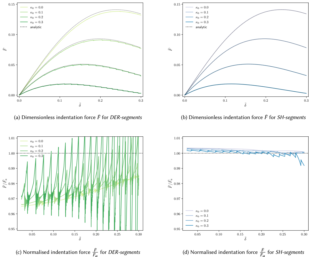
Fig. 5. Curved three-point bending test: noisy force results. Top: Force-indentation curves for DER (left, green) and SH-segments (right, blue), as the natural curvature \kappa_0 is increased (light to dark). Bottom: Normalised curves to better highlight the presence of force jumps in both models, due to segment-based detection.
