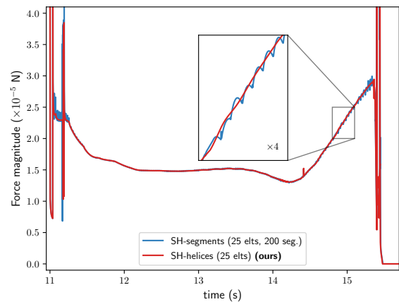
Fig. 12. Hair combing (1) result: comparison between our method and the previous Super-Helices method
