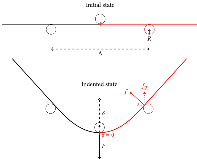
Fig. 3. Classical three-point bending test setup. In our simulations, we consider for simplicity the equivalent “half-system” with an horizontal clamp in the middle, as shown in red. Indentation is obtained by lifting the right-most support.
