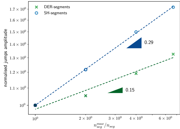
Fig. 20. Evolution of the amplitude of force jumps under refinement: log-log plot of the L_1 norm of the force derivative normalised by its value in the most refined case as a function of the normalised segment length. Segment lengths correspond to 0.1cm, 0.06cm, 0.03cm and 0.015cm for a rod of length 6cm.
