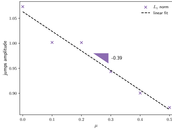
Fig. 26. Curved three-point bending test: analysis of the force discontinuities. L_1 norm of the above curves depict the linear dependency of jump size with respect to friction coefficient at contact.
