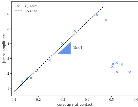
Fig. 13. Force jumps with the actual curvature at contact in the Hair combing (1) scenario. Normalisation of SH-segments by SH-helices .
