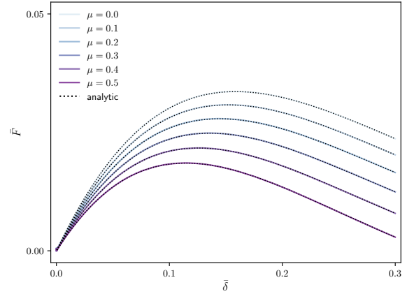
Fig. 22. Curved three-point bending test: noisy force results. Dimensionless force-indentation curves for SH-segments , as the friction coefficient \mu is increased (light to dark).
