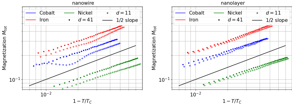
Figure 7: Curie's law. Behavior of M_{\text{tot}}(T) as a function of 1 - T/T_C in logarithmic scale. The materials are represented by different colors: iron (red), cobalt (blue) and nickel (green). The left panel corresponds to nanowires and the right panel to nanolayers, with sizes d = 11 nm (crosses) and d = 41 nm (dots). Each curve was multiplied by a multiplicative factor for easier reading. The black solid lines represent the theoretical 1/2 slope.
