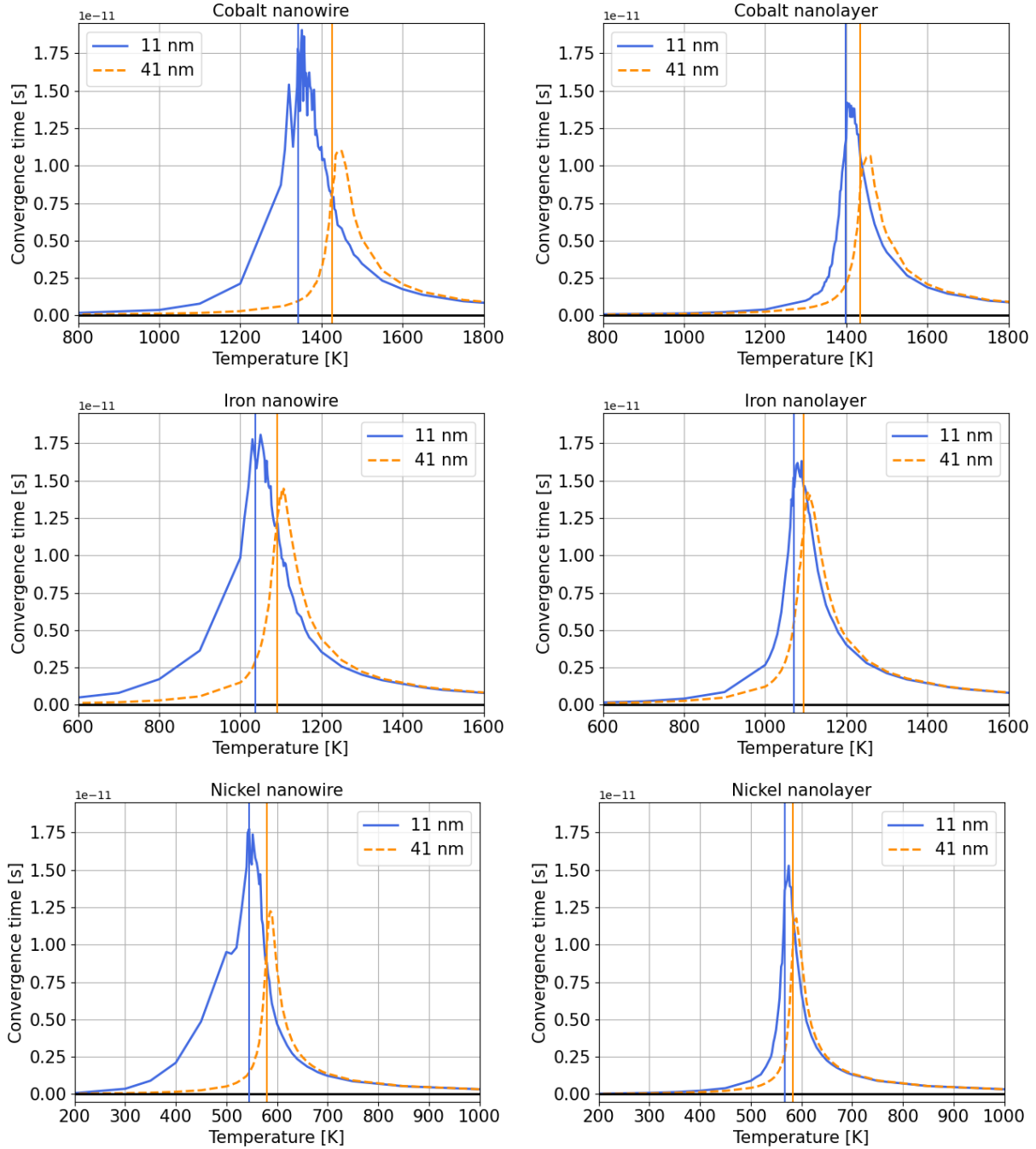
Figure 13: Convergence time t_{\text{conv}} , from Eq. (12), as a function of the temperature for cobalt (top panels), iron (middle panels) and nickel (bottom panels). Left column: nanowire geometry with 6000 \text{ nm} \times d \text{ nm} \times d \text{ nm} ; right column: nanolayer geometry with 600 \text{ nm} \times 600 \text{ nm} \times d \text{ nm} . Two values of d are considered: d = 11 \text{ nm} (blue solid curve) and d = 41 \text{ nm} (orange dash curve). The vertical lines correspond to the numerical Curie temperatures reported in Table 3, for d = 11 \text{ nm} (blue vertical line) and d = 41 \text{ nm} (orange vertical line).
