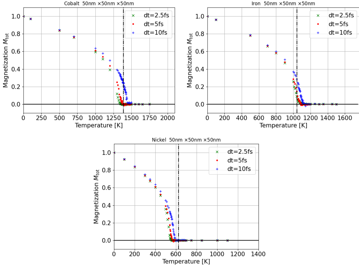
Figure 4: Total magnetization M_{\text{tot}} , from Eq. (10), as a function of temperature, for a cobalt (left), iron (right) or nickel (middle) nanowire with dimensions 50 nm \times 50 nm \times 50 nm. The different symbols stand for different time steps \Delta t = 2.5 fs (green crosses), 5 fs (red circles), and 10 fs (blue crosses). The computational grid size is \Delta x = 1 nm. The black vertical dash-dotted lines represent the bulk Curie temperatures as given in Table 1.
