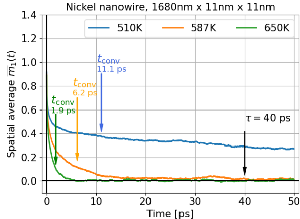
Figure 12: Evolution of the spatially-averaged x component of the magnetic moment \overline{m}_1(t) for a nickel nanowire of cross-section d = 11 nm, for three different temperatures, T = 510 K, T = 587 K and T = 650 K. The corresponding convergence times ( t_{\text{conv}} = 1.9 ps, 6.2 ps, and 11.1 ps) are shown on the figure. We also show the transient time \tau = 40 ps, which is the same for all simulations (time used to average the total magnetization M_{\text{tot}} ).
