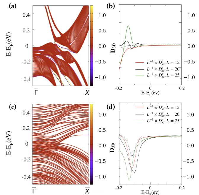
FIG. 9. (Color online) Band structure of a WTe 2 slab containing 25 layers and cut along \hat{z} (a) and \hat{x} (c). For this case the color bar represents the projections on the bottom (-1) and top (+1) layers. (b,d) Corresponding BCD for bulk and slabs containing 15, 20 and 25 layers.
