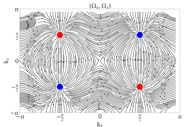
FIG. 1. (Color online) Berry curvature of the Hamiltonian (4) in the (k_x, k_z) plane with k_y = 0 and intrinsic parameters k_0 = \frac{\pi}{2} , m = 2 , t_x = \frac{1}{2} , \gamma = 1 and t = 1 . Note that the Berry curvature of the two-band model is not sensitive to the value of \gamma [51]. The solid lines represent the Berry curvature vector field (\Omega_x, \Omega_z) , whereas the blue (red) dots represent the local positive (negative) divergencies taking place at the Weyl nodes.
