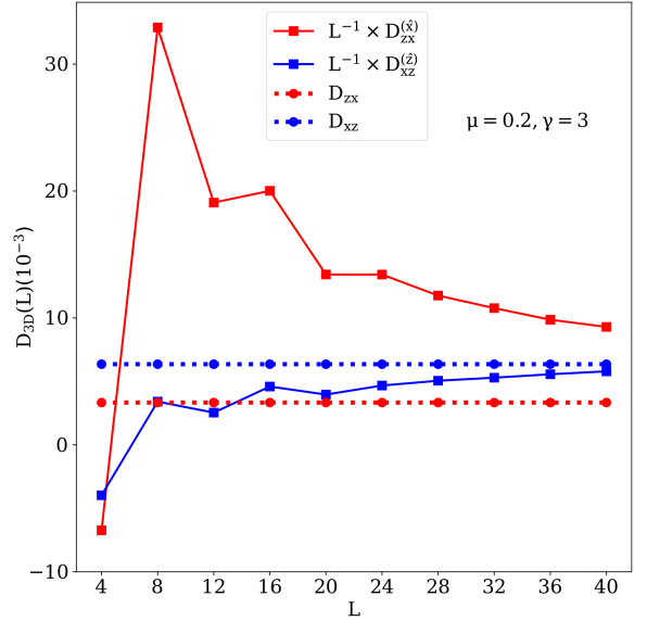
FIG. 6. (Color online) Thickness dependence of the BCD in a type II WSM for the \hat{z} -cut (blue) and \hat{x} -cut (red), as compared to the bulk values (dashed lines). The \hat{x} -cut shows a very strong deviation from the bulk value at small thicknesses, illustrating the importance of the surface states in this case.
