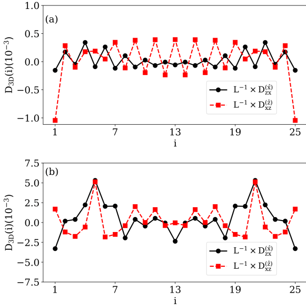
FIG. 5. (Color online) Layer dependent contribution for the BCD normalized by the number of layers (in this case, L = 25 ). We show the tomography for a type I WSM with \gamma = 1 in (a) and for a type II WSM with \gamma = 3 in (b).
