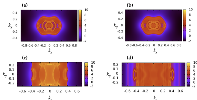
FIG. 8. (Color online) WTe 2 density of states at Fermi level, projected on the bulk (a,c) and top surfaces (b,d) for a slab geometry containing 25 layers. Panels (a,b) correspond to a cut along \hat{z} whereas panels (c,d) correspond to a cut along \hat{x} .
