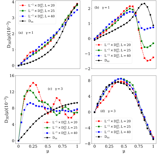
FIG. 11. (Color online) Dependence of the BCD as a function of the chemical potential for the (a, c) x -cut and (b, d) z -cut, for type I ( \gamma = 1 ) and type II ( \gamma = 3 ) WSM.
