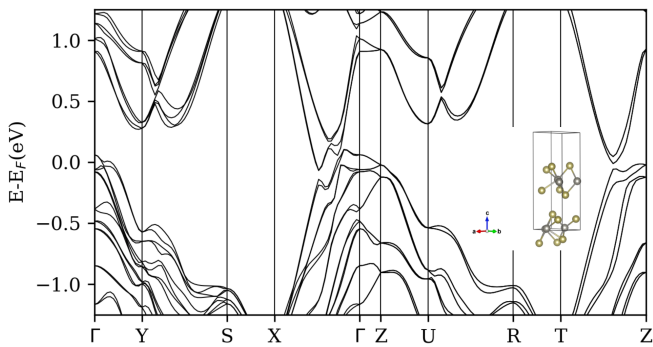
FIG. 7. (Color online) Bulk band structure of WTe 2 type II WSM obtained from density functional theory simulations. The inset displays the unit cell.
