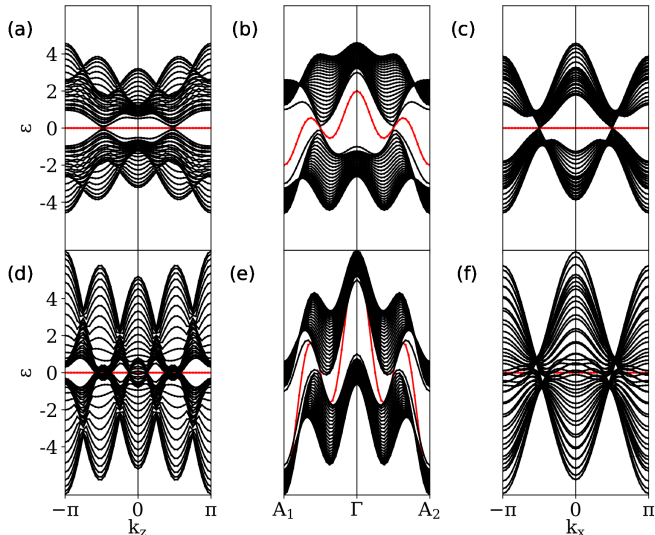
FIG. 2. (Color online) Band structures of the WSM slab of 25 layers, with \gamma = 1 (a-c) and \gamma = 3 (d-f) along the high symmetry path of the cubic lattice for different cuts: (left panels) \hat{x} for k_y = 0 and k_z \in [-\pi, \pi] , (center) \hat{y} along the path A_1 = (-\pi, 0, -\pi) \rightarrow \Gamma = (0, 0, 0) \rightarrow A_2 = (\pi, 0, \pi) and (right) \hat{z} for k_y = 0 and k_x \in [-\pi, \pi] . The central panels clearly displays type I (b) and type II (e) Weyl cones. The surface states at the top and bottom surfaces are represented with a solid red line. The flat red bands in (a), (c), (d) and (f) are surface states at zero energy that are highly localized at the corresponding surfaces.
