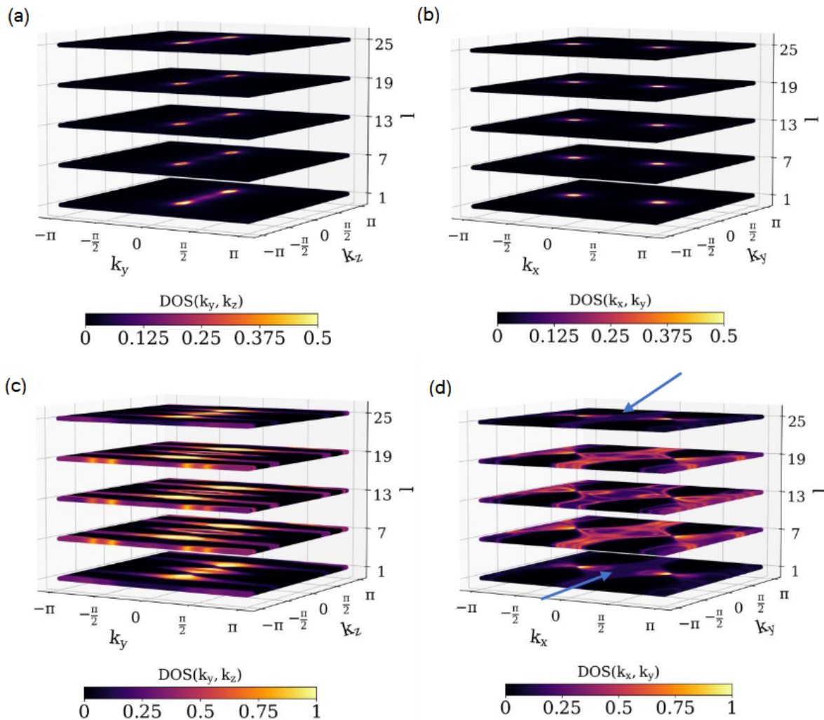
FIG. 3. (Color online) Projected density of states (DOS) for (a, c) \hat{n} = \hat{x} and (b, d) \hat{n} = \hat{z} as a function of the momentum coordinates for selected layers l for the type I ( \gamma = 1 ) (a, b) and type II ( \gamma = 3 ) phase (b, d). For the \hat{x} -cut in the type I phase (a), the Weyl nodes dominate in the bulk and get connected by degenerate Fermi arcs at the surface, whereas in the type II phase (c), large trivial Fermi pockets appear across the slab. For the \hat{z} -cut in the type I phase (b), the Weyl nodes remain disconnected across the slab, whereas in the type II phase (d), trivial Fermi pockets dominate in the bulk with track states and projected Weyl nodes at the surface. The track states' projections are centered around k_x = 0, \pm\pi , which are indicated with blue arrows on each corresponding layer.
