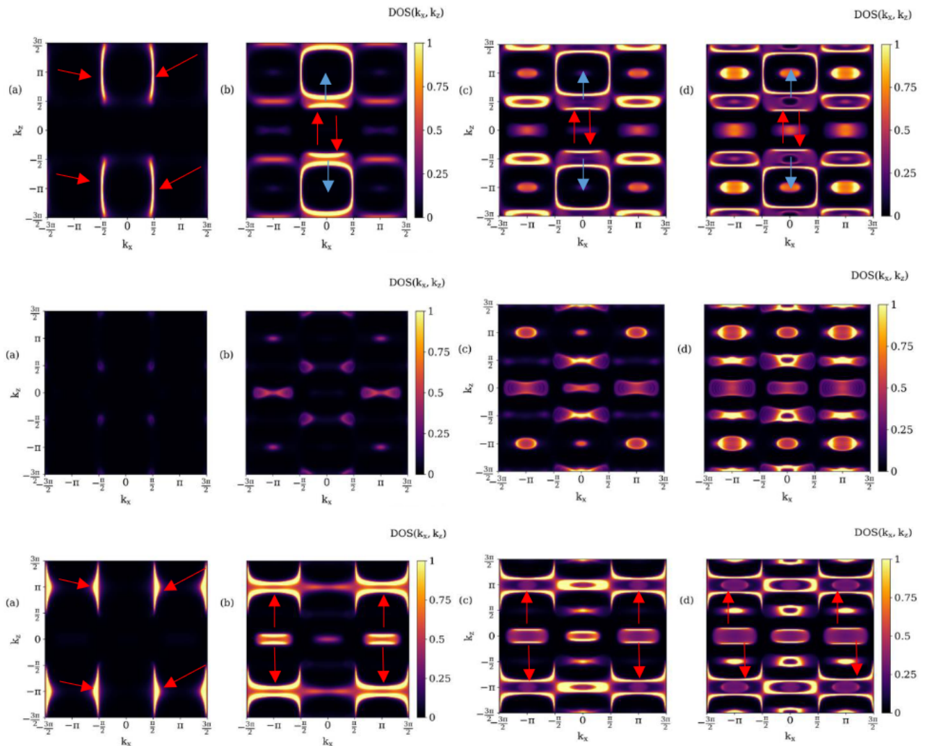
FIG. 10. (Color online) Layer-resolved density of states of the topmost (top panels), central (middle panels) and bottommost (bottom panels) surface of a system with 25 layers and \mu = 0.2 . The red arrows indicate the Fermi arcs, and the blue arrows point to the center of the track states. Finally, indexes (a-d) show the cases \gamma = 1, 2, 2.5, 3 , respectively, i.e., tracking the transition from type I to type II WSM. The mismatch between the top and bottom surfaces is in agreement to what is reported in [51], and we assign this behavior to the absence of mirror symmetry along \hat{y} in the original Hamiltonian given by Eq. (4).
