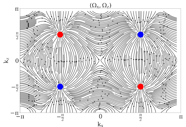
FIG. 1. (Color online) Berry curvature of the Hamiltonian (4) in the (k_x, k_z) plane with k_y = 0 and intrinsic parameters k_0 = \frac{\pi}{2} , m = 2 , t_x = \frac{1}{2} , \gamma = 1 and t = 1 . Note that the Berry curvature of the two-band model is not sensitive to the value of \gamma [51]. The solid lines represent the Berry curvature vector field (\Omega_x, \Omega_z) , whereas the blue (red) dots represent the local positive (negative) divergencies taking place at the Weyl nodes.
