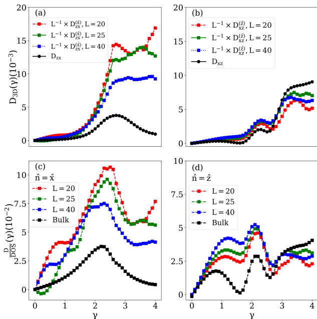
FIG. 4. (Color online) BCD components as a function of the tilting parameter \gamma for slab and bulk systems. (a) Slab ( D_{zx}^{\hat{x}}/L ) and bulk ( D_{zx}^{3D} ) components for the \hat{x} -cut, for different slab thicknesses. (b) Slab ( D_{xz}^{\hat{z}}/L ) and bulk ( D_{xz}^{3D} ) components for the \hat{z} -cut, for different slab thicknesses. (c, d) Corresponding ratio between the BCD coefficient and the corresponding density of states for bulk and slab systems for the \hat{x} -cut (c) and \hat{z} -cut (d).
