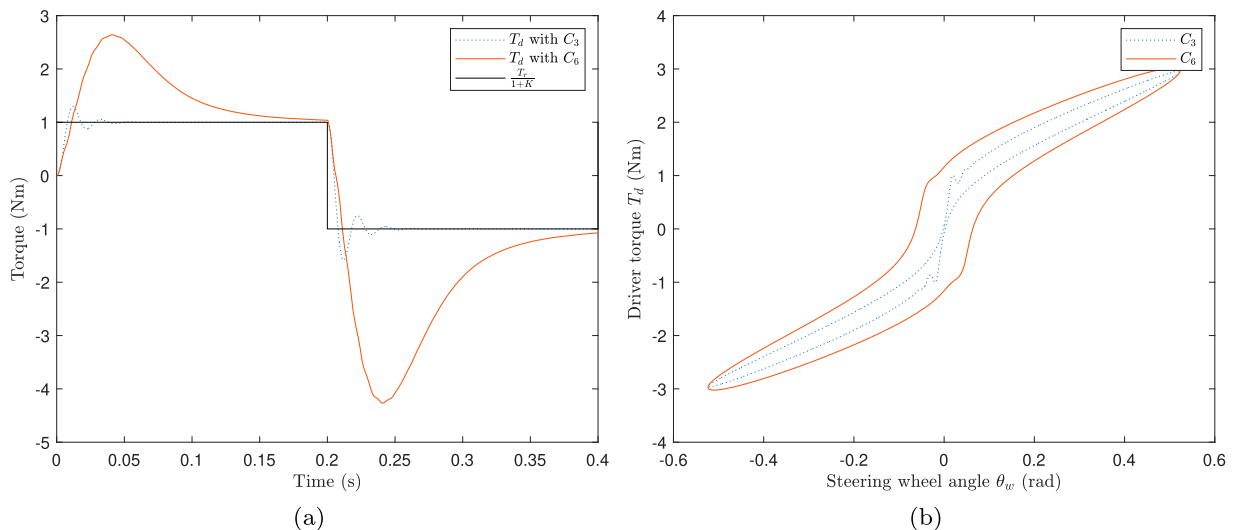
Figure 16. Driver comfort assessment tests for \sigma_p = 1.35 Nm.s/rad, with a constant delay \tau = 1.5 ms. (a) Driver torque for a road torque input given by a square signal. (b) Hysteresis curve to assess the steering feel.
