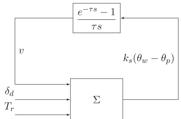
Figure 8. LFT representation of the EPS system.
