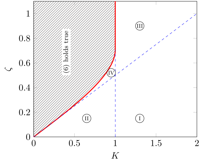
Figure 5. The four different cases where (6) does not hold true.
