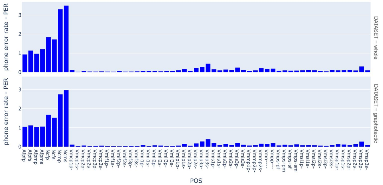
Figure 4. PER for each paradigm cell of the three POSs A, N, and V, and for the two datasets.
