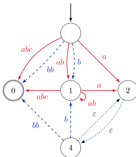
■ Figure 1 Automaton corresponding to keyboard \{\leftarrow\text{abc}, \leftarrow^4\text{bb}\} .
