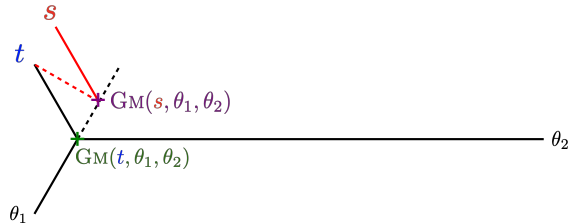
Figure 1: A simple example where the geometric median fails to be strategyproof. This example is easy to analyze in the limit where \theta_2 is infinitely far on the right, in which case its pull is always towards the right. Since the unit pulls of all voters must cancel out, there must be a third of a turn between any two unit pull. This shows why, as the strategic voter reports s rather than their target vector t , the geometric median moves up the dotted line, closer to t .
