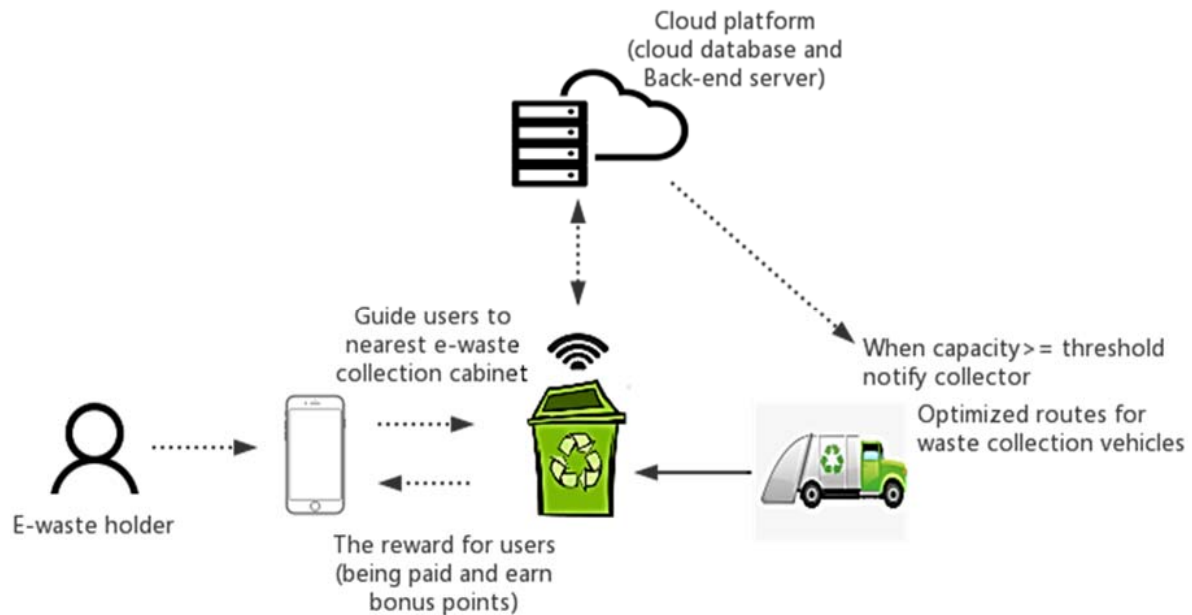
Figure 2 – The architecture of IoT-based e-waste collection platform
