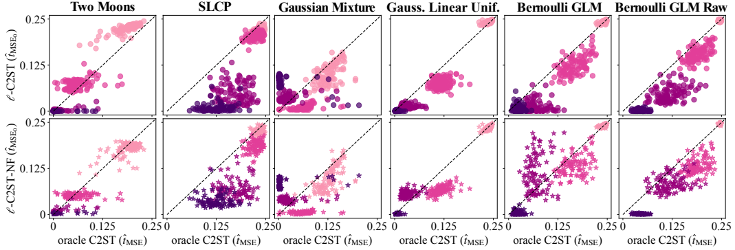
(b) 100 observations (generated via sbibm package)
