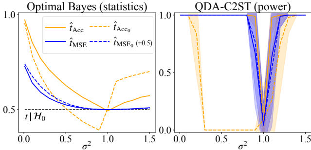
Figure 1: Results for the C2ST framework when p = \mathcal{N}(0, \mathbf{I}_2) and q = \mathcal{N}(0, \sigma^2 \mathbf{I}_2) . Left panel portrays the test statistics for the optimal Bayes classifier and the right panel shows the test's empirical power with QDA. Single-class accuracy test ( \hat{t}_{\text{Acc}_0} ) fails to detect when p \neq q but \hat{t}_{\text{MSE}_0} behaves correctly.
