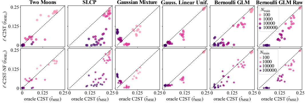
(a) 10 observations (same as in benchmark experiment in Figures 2 and 5)
