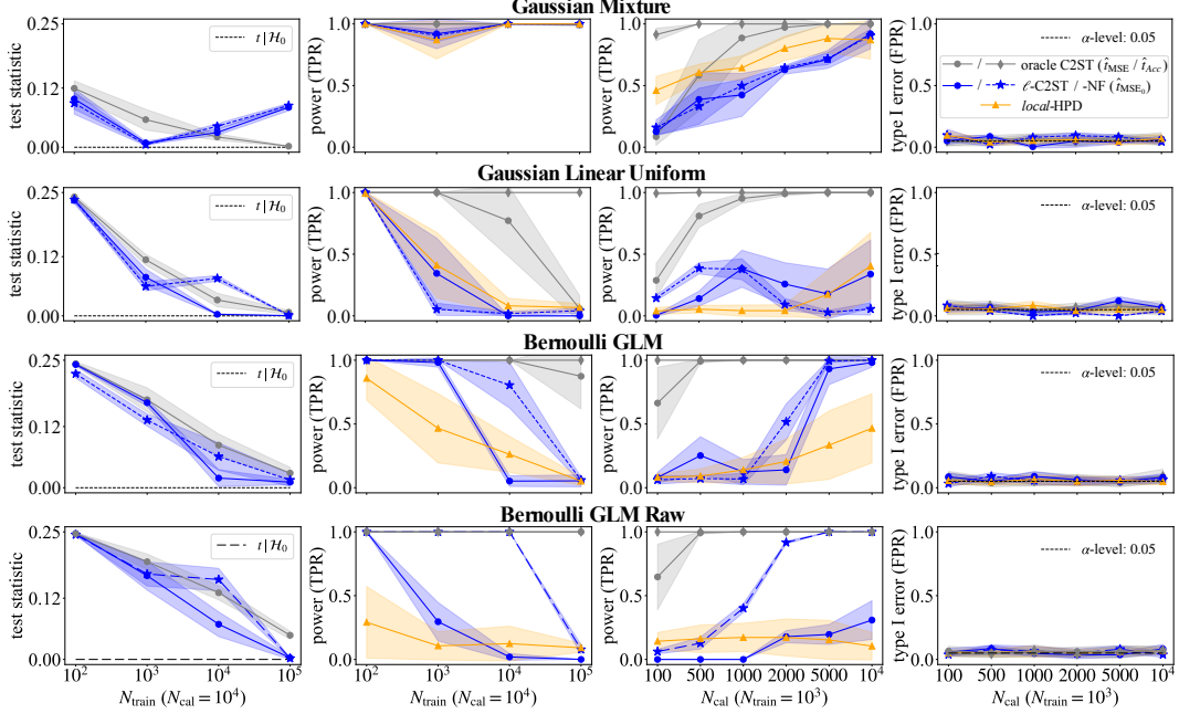
Figure 5: Results on additional sbibm benchmark examples using the same experimental setup as for Figure 2 in Section 4 (50 test runs, mean / std over 10 different reference observations).
