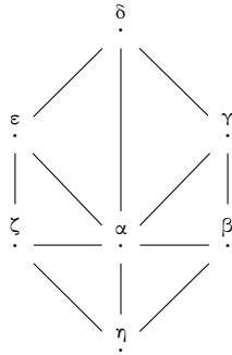
Figure 8.1: Granular spin network: it is a loop-like graph. There are ( spin network ) nodes, i.e. points acting as quanta of space, and links, for a (\alpha\text{-}\beta\text{-}\gamma\text{-}\delta\text{-}\epsilon\text{-}\zeta\text{-}\eta) -nodal lump of space. Note that \alpha\beta\gamma order is chosen with personal preference: there is no rotational privilege, because there is no spatial order ab initio
