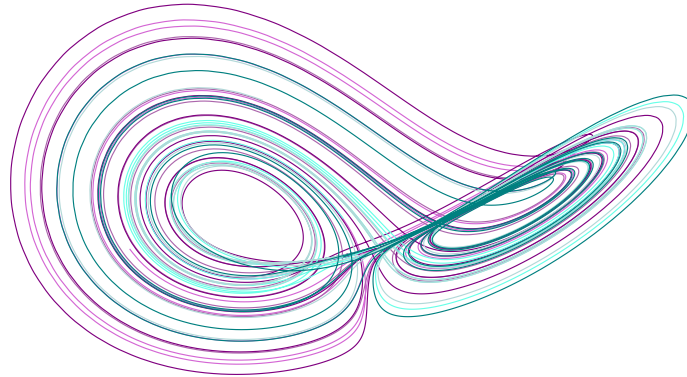
Figure 15.1: Lorenz attractor via Euler method in 6 strokes, with localsigma[Pr] = 3, localrho[Ra] = 26.5, localbeta = 1, and return{sigma * (y - x), -x * z + rho * x - y, x * y - beta * z} . The total number of orbits starting from various initial points is six: ● ● ● ● ● ●
