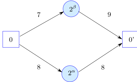
Figure 7 The solution with T^s(\xi) = 16 is infeasible
