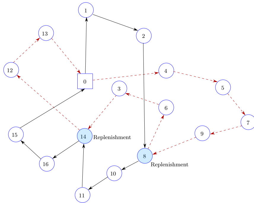
Figure 2 A feasible solution of a TSPBR instance with 16 customers
