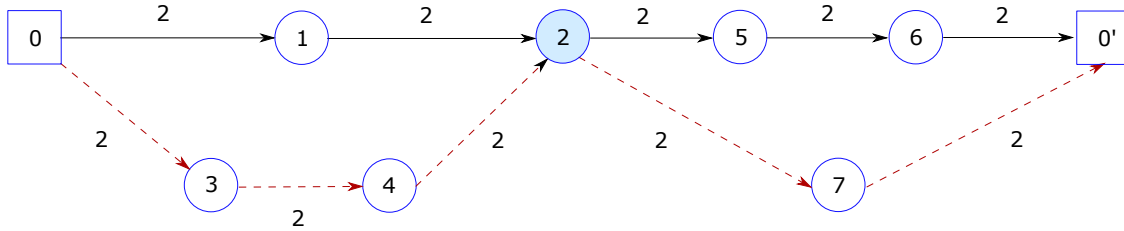
Figure 3 A solution with two operations and \tilde{\mathcal{T}}^s(\xi) = 16
