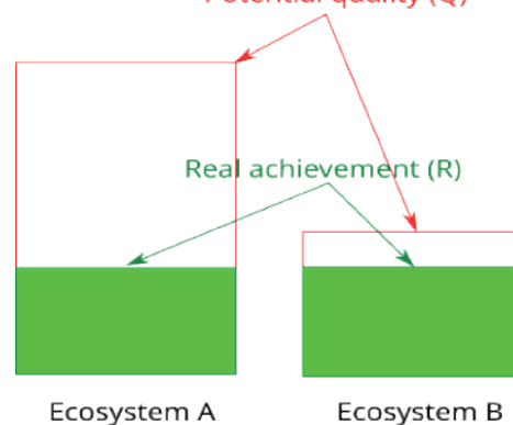
Figure 7: The health of an ecosystem can be assessed by measuring the difference between a potential quality and its realisation. For example, here, if we take the number of species as the estimator, ecosystem B would be healthier than ecosystem A, although it has the same number of species, because it realises a much larger fraction of its potential. Based on Kibblewhite (2008) and Alain Brauman about soil healths, modified.
