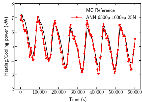
Fig. 6: Las Vegas, 2019 Summer week: Monte Carlo simulation in black color (reference solution), interpolation using TMY with the FANN in red color. Configuration with photovoltaic field, green roof layer.
