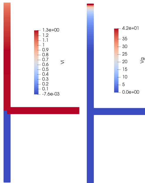
Figure 10: Liquid and gas superficial velocities ( \text{m}\cdot\text{s}^{-1} ) at final time for the cross flow thermal well test case.
