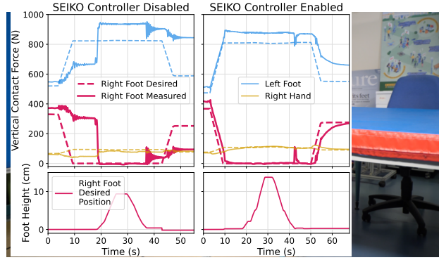
Figure 4. Comparison of contact switch trials with and without SEIKO Controller. Initially, both feet and right hand are in contact. The operator teleoperated the robot to disable the right foot contact, lift the foot, and re-establish contact. Vertical contact forces \lambda^d, \lambda^{read} (top row) and the desired vertical position of the right foot X_{right\ foot}^d (bottom row) are displayed.
