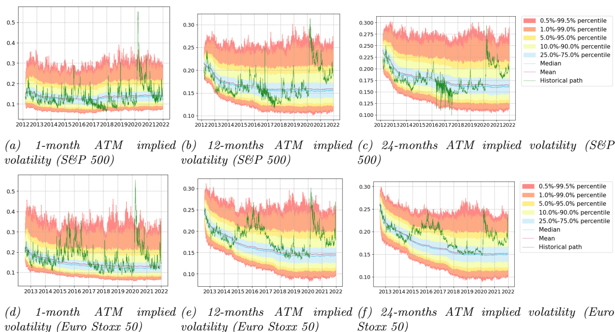
Figure 23: Quantiles envelopes of the ATM implied volatility for several maturities.
