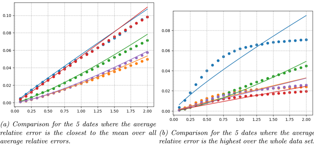
Figure 14: Comparison of the S&P 500 ATM total variances (dots) with the fitted parametric form T \mapsto aT^p (lines) for some dates (each color corresponds to one date).
