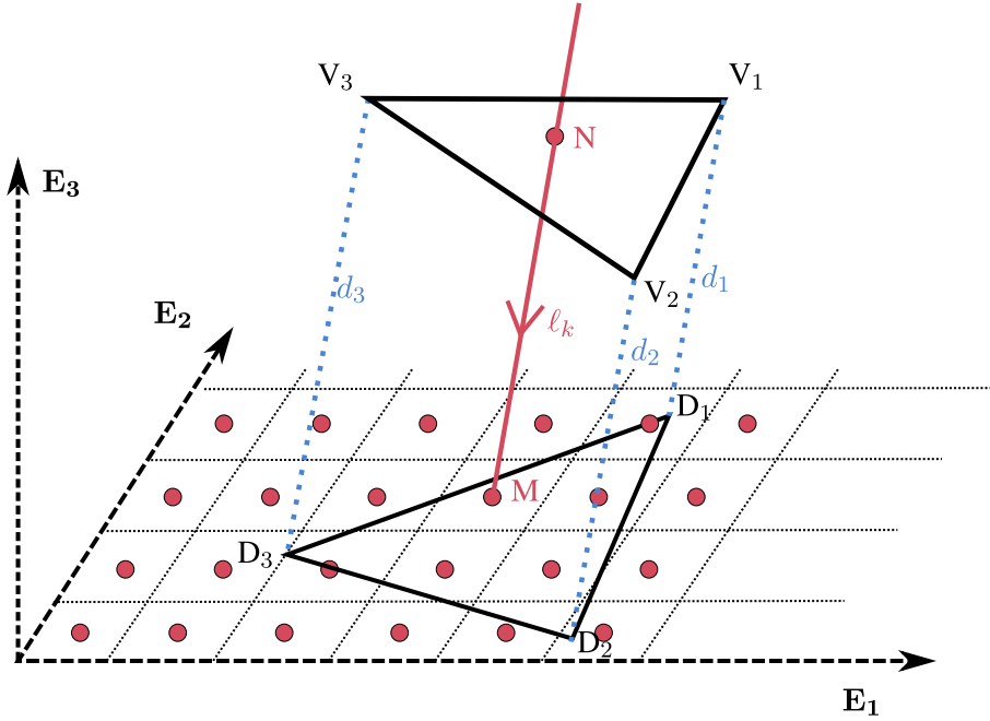
Figure 2: Illustration of rasterization technique, projections (D_0, D_1, D_2) of the vertices of the triangle (V_0, V_1, V_2) .
