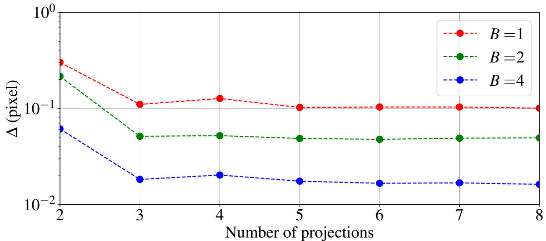
Figure 5: Measurement error \Delta as a function of the number of projections for different binning factor B .
