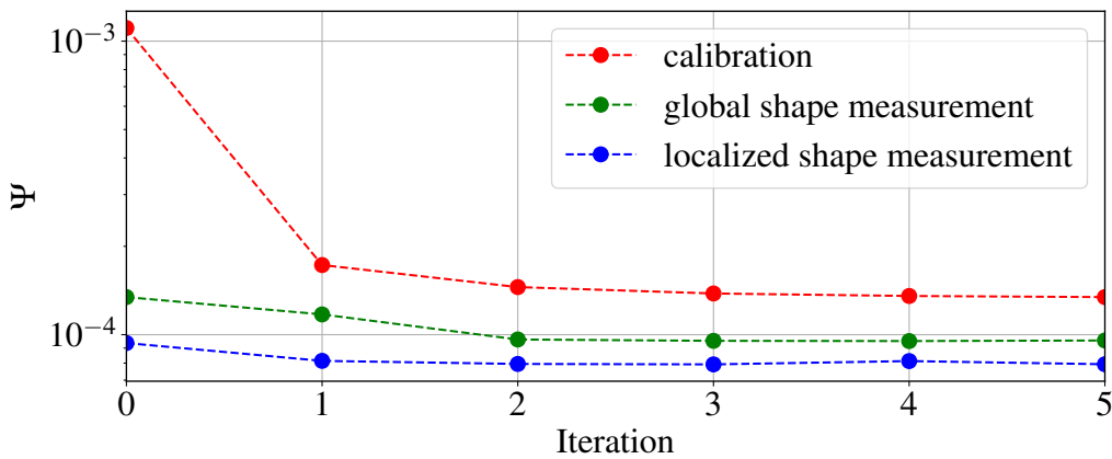
Figure 11: Evolution of the cost function \Psi during the iterative registration process
