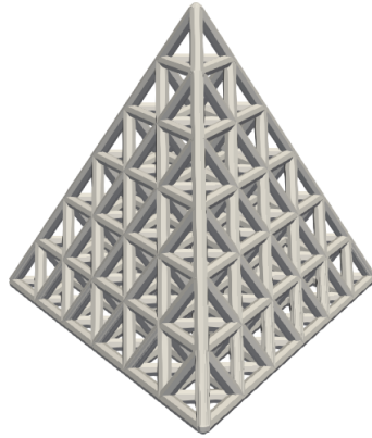
Figure 3: CAD model of the tetrahedral lattice material
