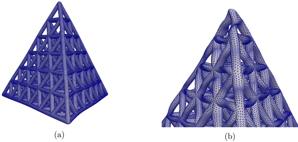
Figure 12: (a) \times 10 magnified displacement from the initial CAD model after the global 35 RBF points measure. (b) \times 2.5 magnified displacement from the initial CAD model after the local 165 RBF points measure.
