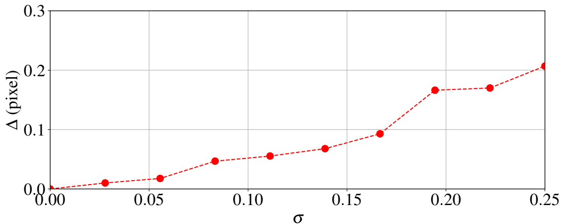
Figure 7: Measurement error as a function of the noise level
