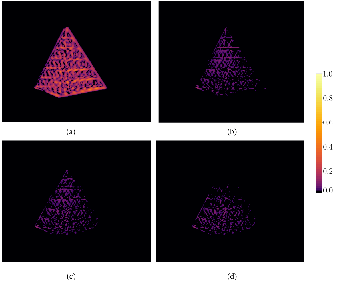
Figure 10: Error maps \delta_\theta for \theta = 63^\circ after (a) manual setup, (b) calibration, (c) 35 RBF control points measurement, (d) 165 RBF control points around the upper vertex measurement.
