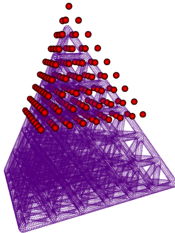
Figure 9: Initial location of the 165 RBF control points (red) for the second step
