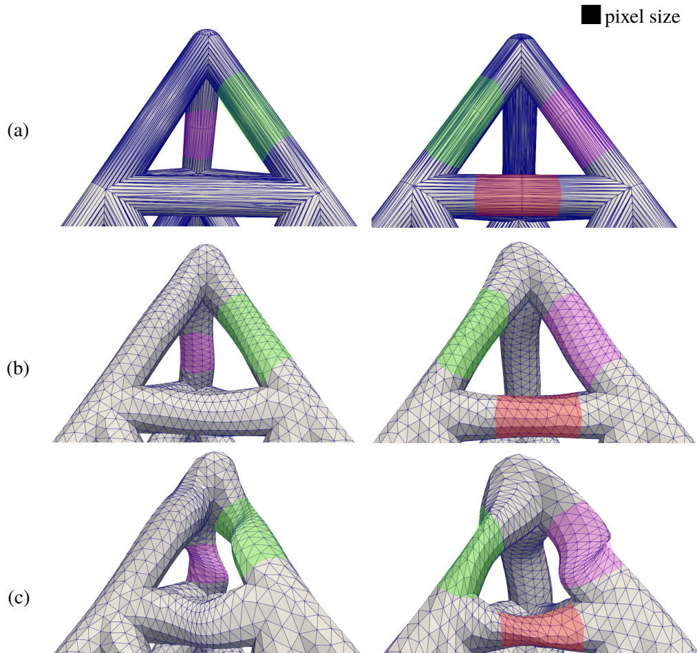
Figure 13: Upper vertex detail. (a) mesh used for printing. 3D printing connection areas are colored. (b) true scale displacement from the initial CAD model after the global 35 RBF points measure (c) \times 2.5 magnified displacement from the initial CAD model after the local 165 RBF points measure
