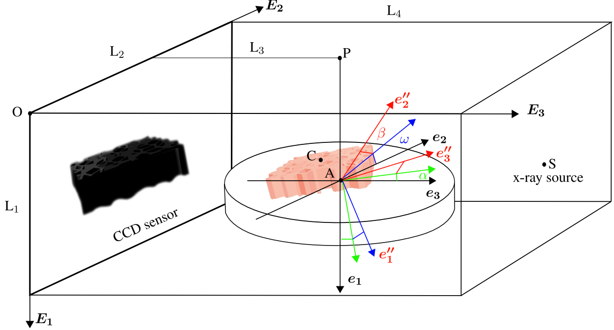
Figure 1: tomograph geometry (in \theta = 0 case)
