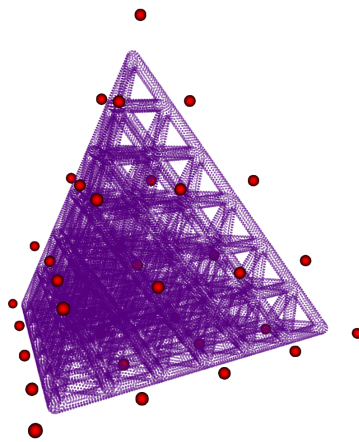
Figure 4: Reference part and the 35 RBF control points (red)
