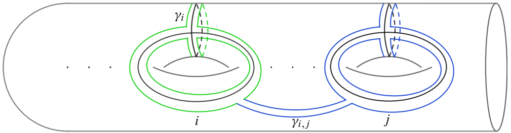
Figure 4: Curves \gamma_i and \gamma_{i,j} .
