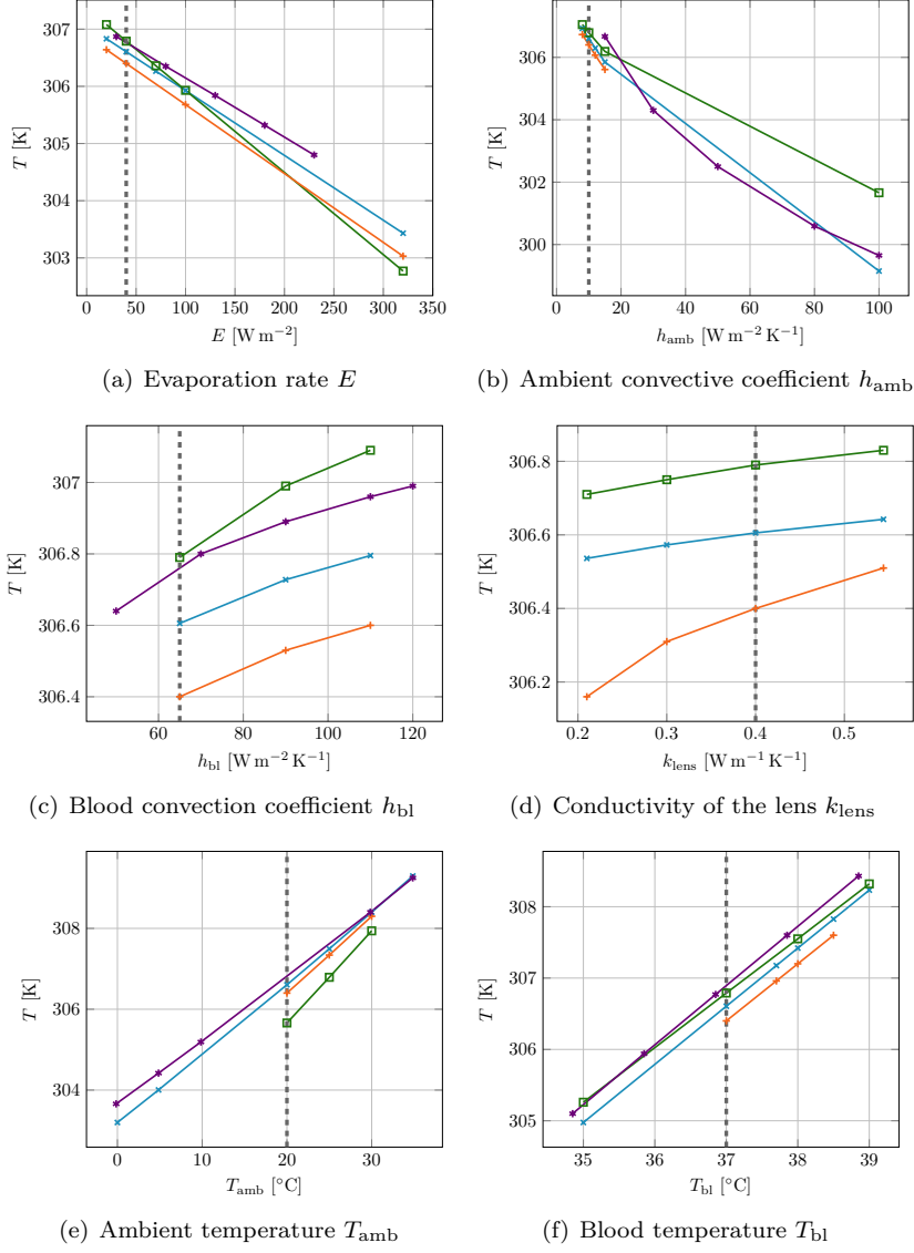
Figure 11: Results of the DSA for the 6 parameters studied, among previous studies from the literature (markers \times \mathcal{E}_{NL}(\mu) , \square [Ng 06], + [Sco88], * [Li+10]). The vertical dashed line corresponds to the baseline value of the parameter.
