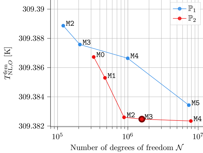
Figure 4: Temperature at the center of the cornea computed with the high-fidelity model \mathcal{E}_{\text{NL}}(\bar{\mu}) , depending on the level of refinement of the mesh.
