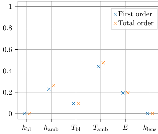
(a) Output T_O .
