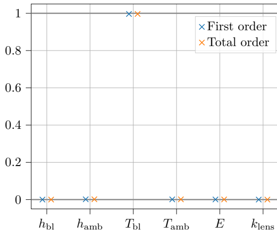
(e) Output T_{D_1} .
