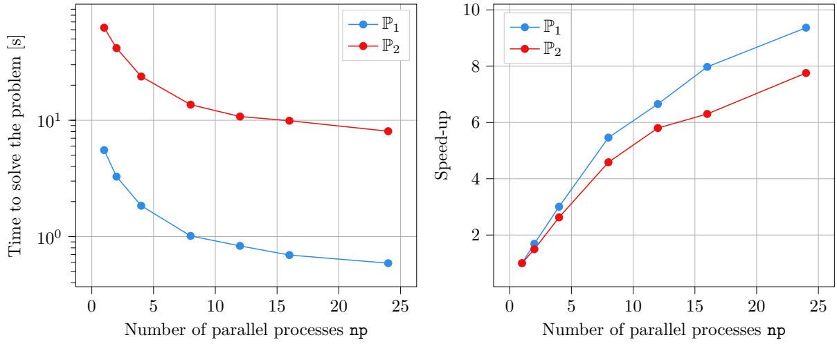
Figure 5: Time of execution to run \mathcal{E}_L^{\mathcal{N}}(\bar{\mu}) and corresponding speed-up, for an increasing number of parallel processes. Simulations are performed on the M3.
