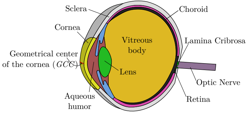
Figure 1: Geometrical model of the human eye.
