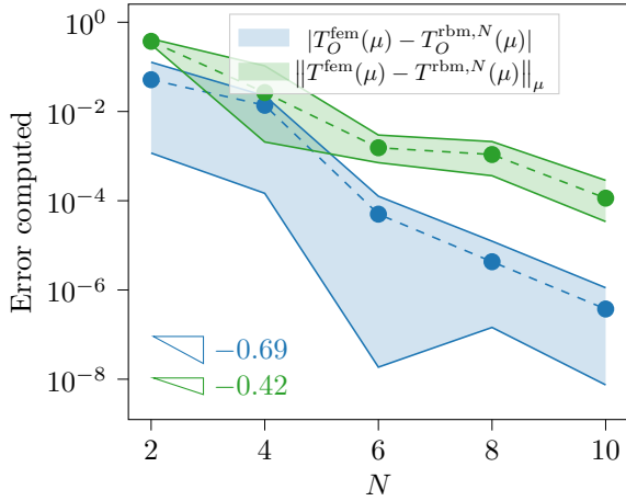
(b) Convergence of the errors on the field and the output on point O , for \mu \in \Xi_{\text{test}} , for various reduced basis sizes. The maximal, minimal, and mean values are represented.
